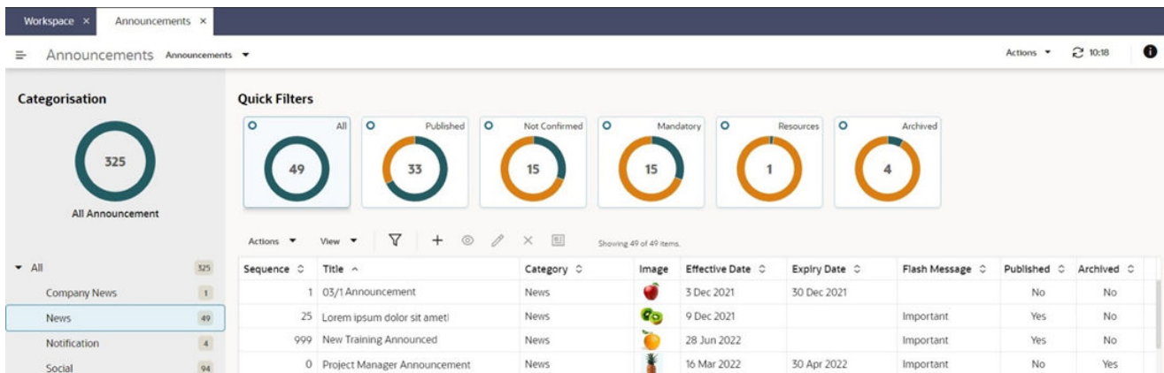
Figure 4-3 Announcements Page
