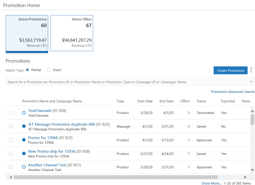
Figure 5–171 Promotion Home
