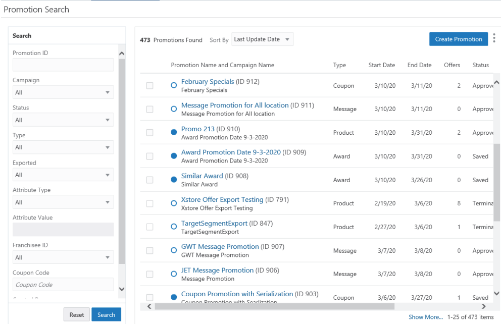
Figure 5–172 Promotion Search
