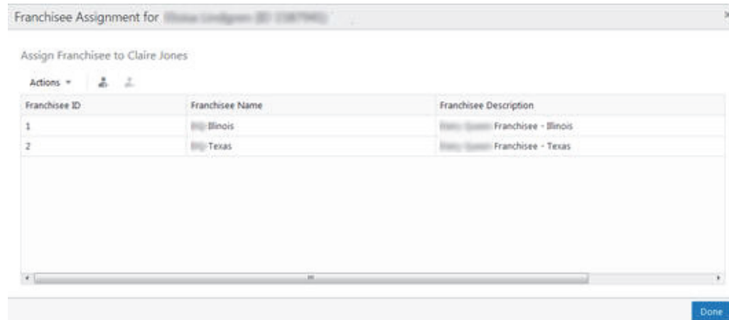
Figure 4–62 Franchisee Assignment
