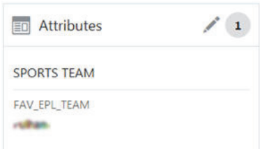
Figure 4–19 Customer Attributes
