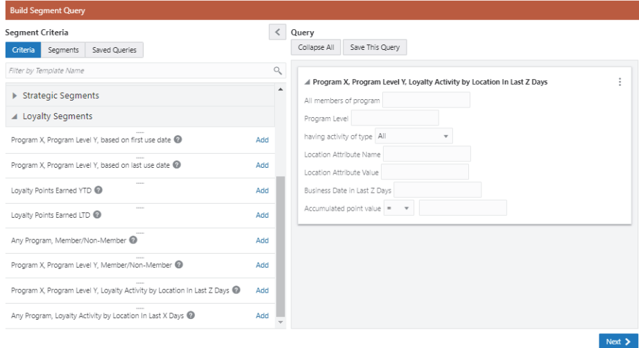
Figure 7-18 Added Criteria
