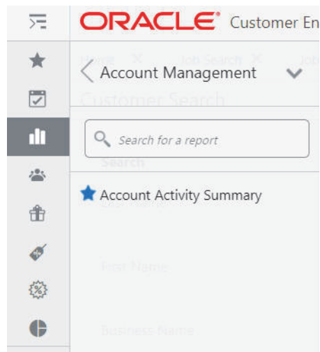
Figure 1–9 Favorite
