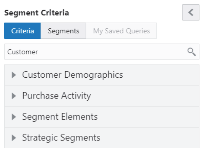
Figure 7–15 Criteria - Filtered
