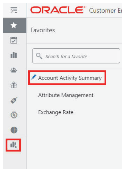
Figure 1–15 Pinned Favorites
