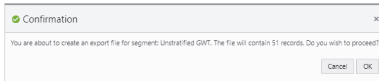
Figure 7–61 Export Confirmation
