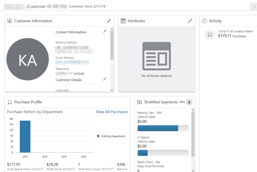
Figure 4–1 Customer Dashboard
