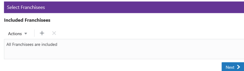
Figure 5–137 Franchisees Tab
