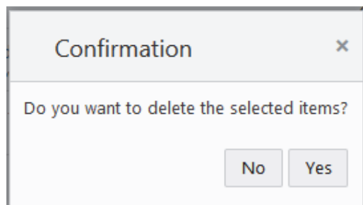
Figure 8–18 Confirmation Prompt
