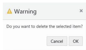
Figure 4–56 Warning Message
