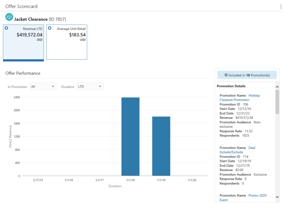
Figure 6–65 Offer Scorecard
