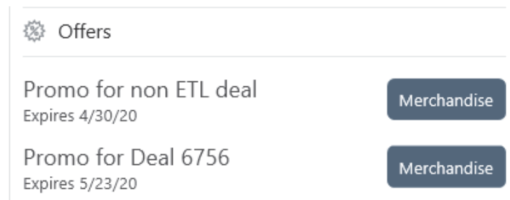
Figure 4–44 Offers
