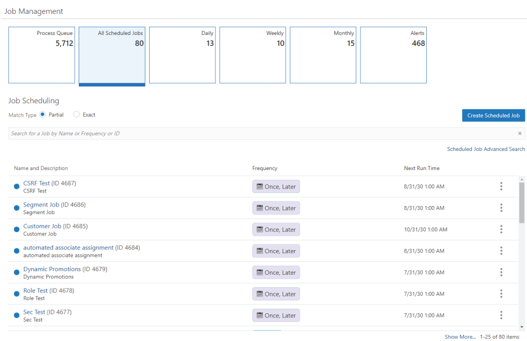
Figure 10–12 Job Home
