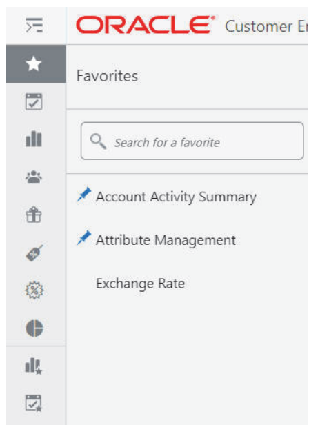
Figure 1–10 Favorites
