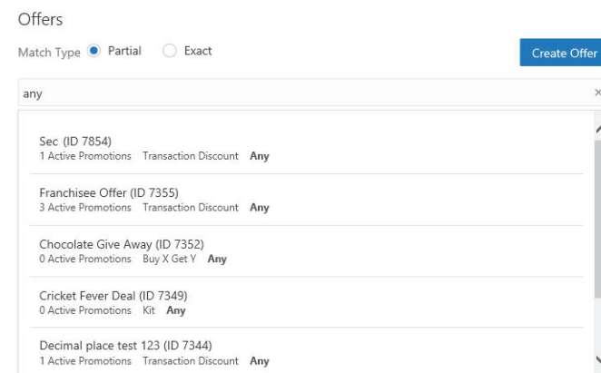
Figure 6–2 Offers
