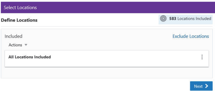
Figure 5–73 Locations Tab
