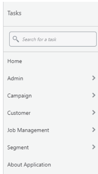
Figure 1–2 Task List
