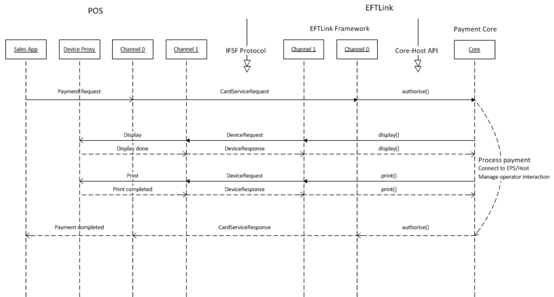
Figure 3-2 Message Flow
