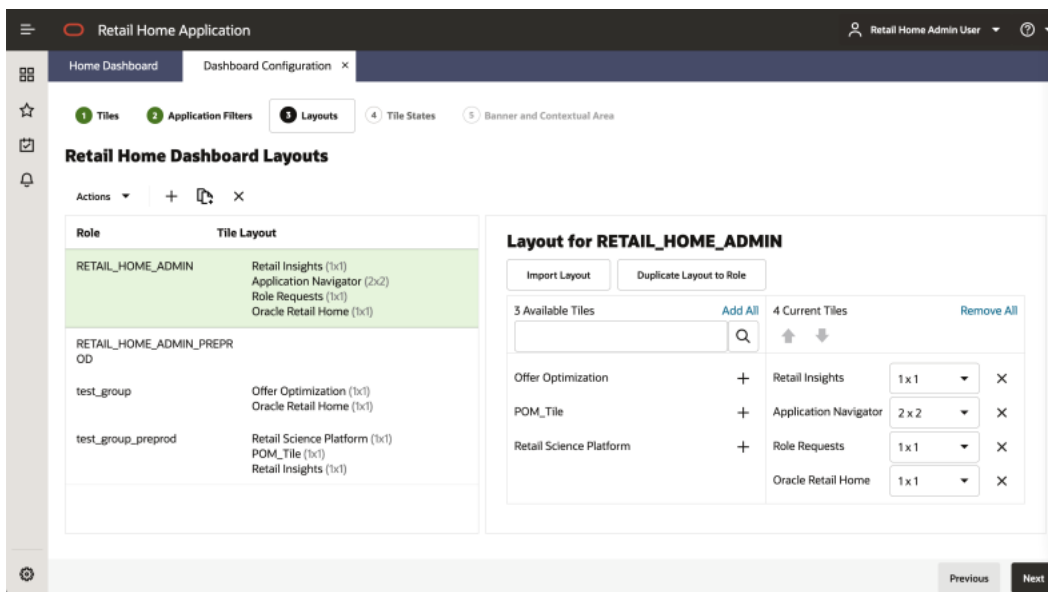
Figure 2-15 Mapping Table for Role and Application Tiles
