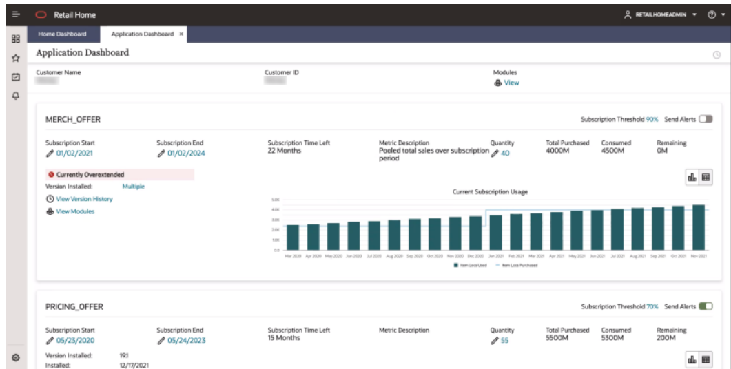
Figure 4-1 Application Dashboard Page
