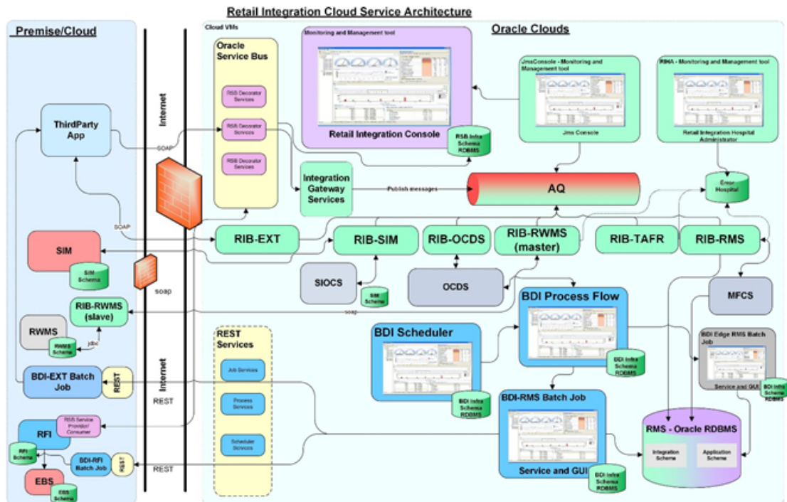
Figure 2-2 RICS Architecture
