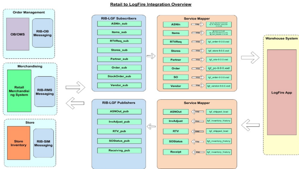
Figure 2-7 Retail to LogFire Integration Overview
