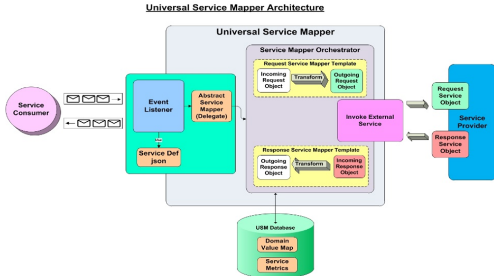
Figure 2-5 USM Architecture
