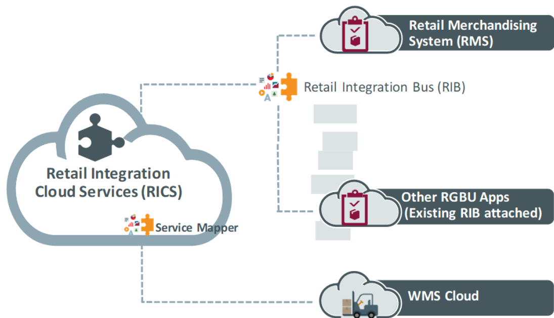
Figure 2-6 WMS-RICS Mappings
