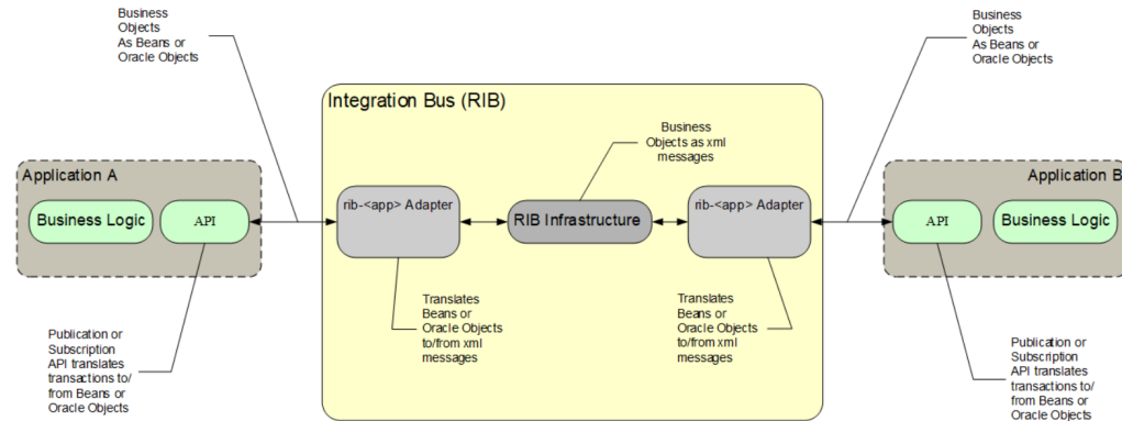
Figure 3-1 RIB Integration Responsibilities
