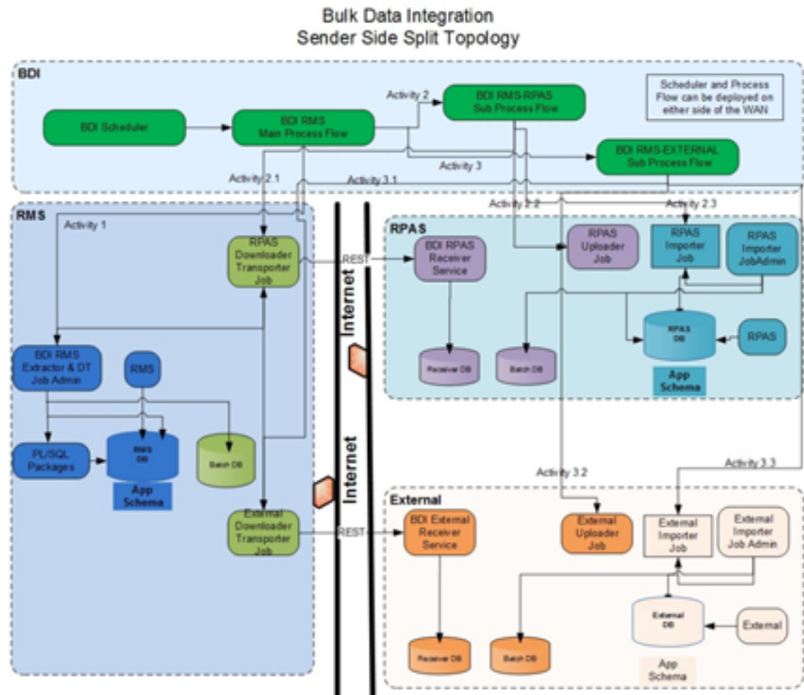
Figure 8-2 Sender Side Split Topology
