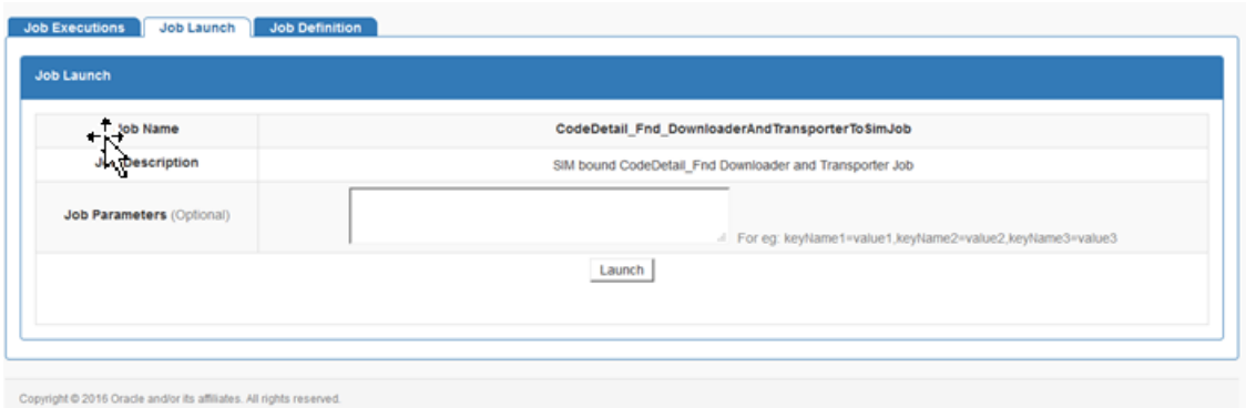
Figure 5-3 Job Launch
