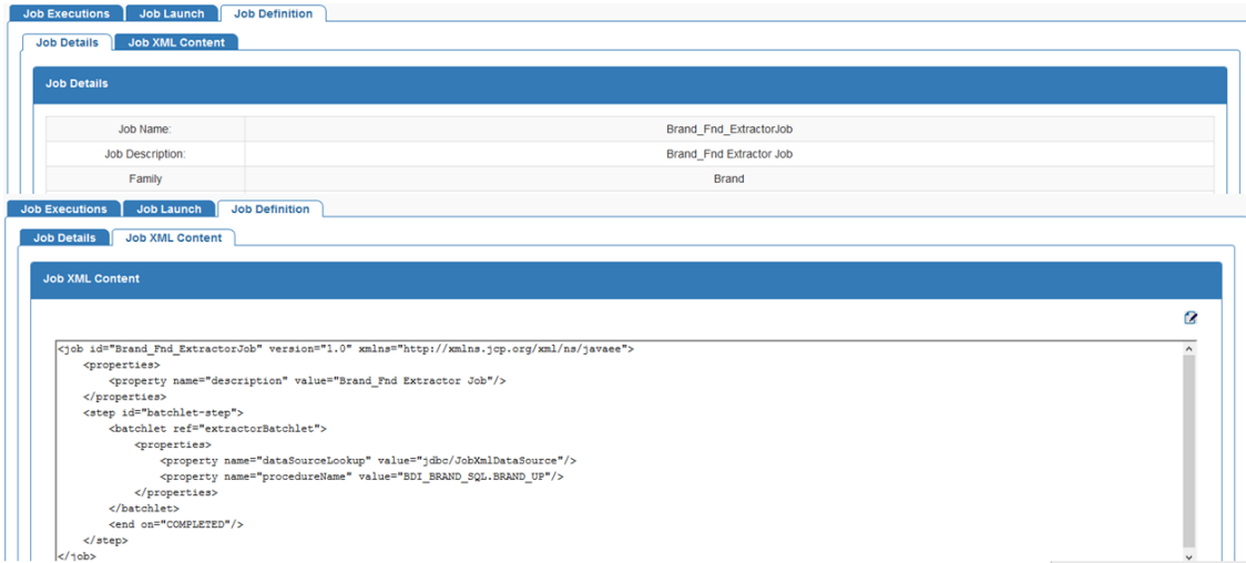
Figure 5-4 Job Details
