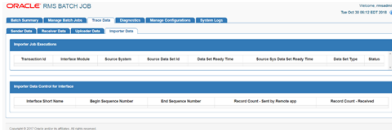
Figure 5-9 Importer Data
