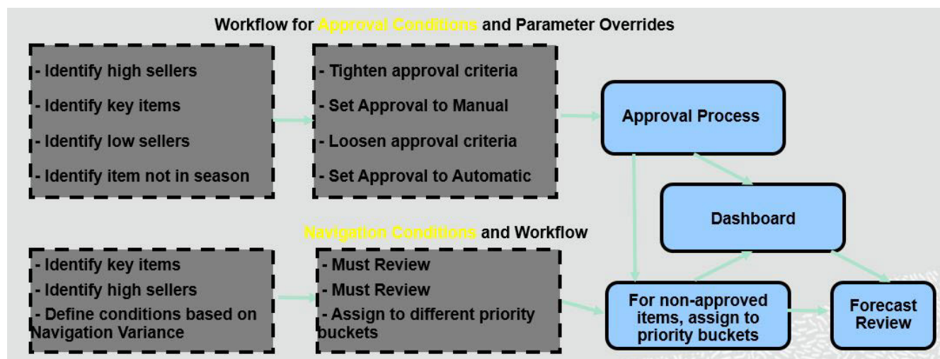
Figure C-3 Rule Conditions
