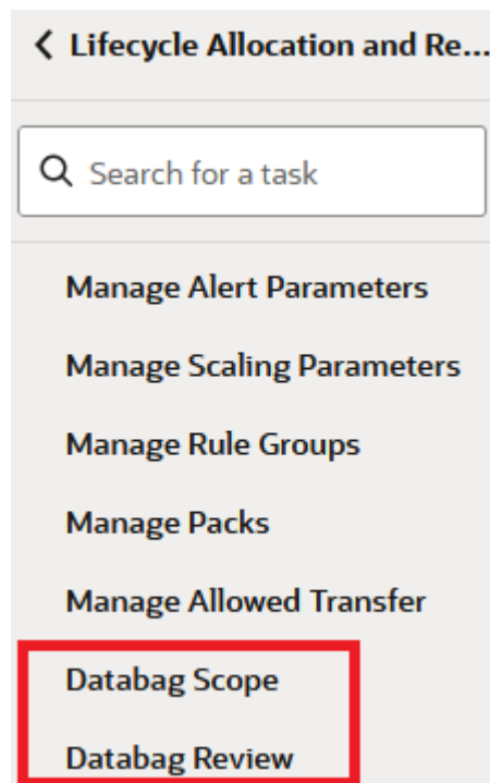
Figure 15-5 Databags Wizard
