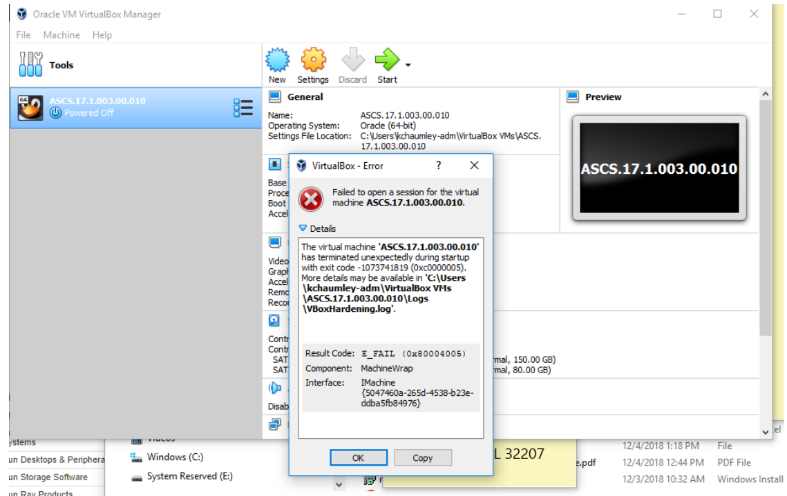
Figure 3-20 VirtualBox Error
