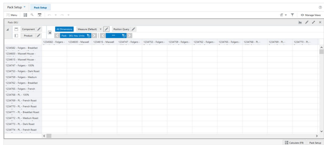
Figure 17-6 Pack-SKU View
