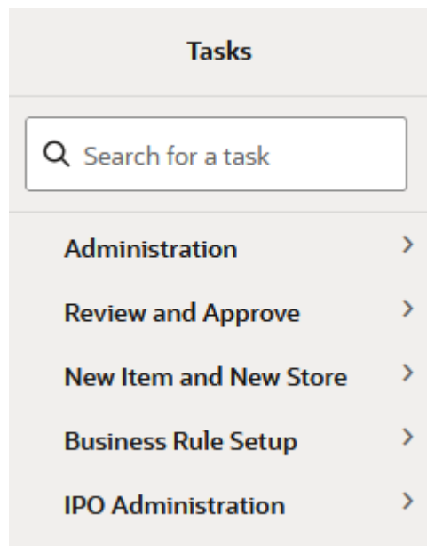
Figure 3-11 Task Module
