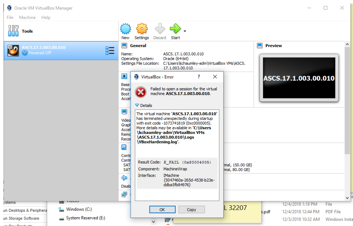
Figure 3-20 VirtualBox Error
