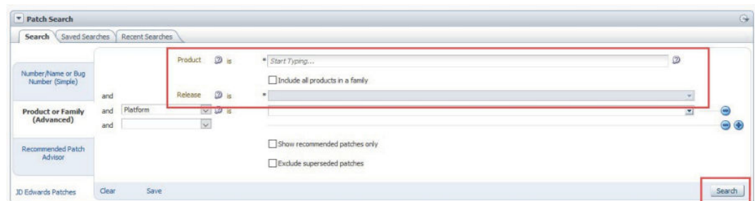
Figure 2-1 Patch Search
