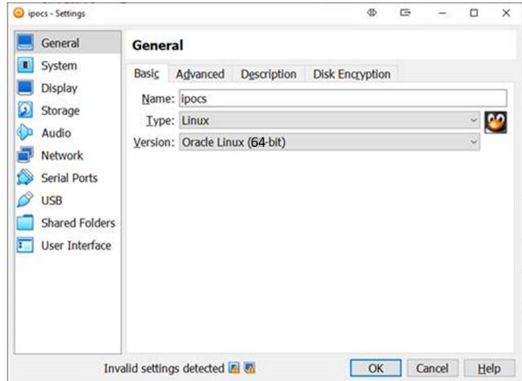
Figure 3-7 Basic Tab
