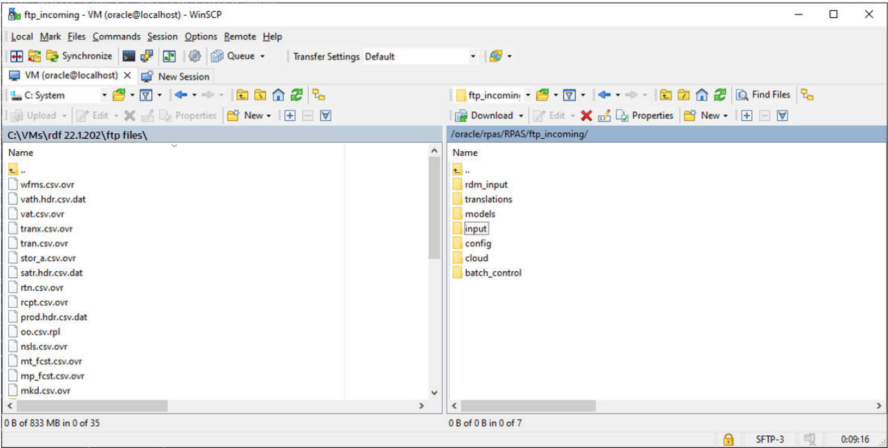
Figure 3-18 FTP Locations
