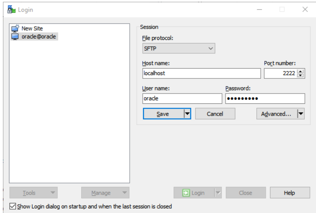
Figure 3-17 Sharing Files
