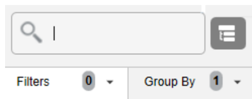
Figure 7-4 Search Bar
