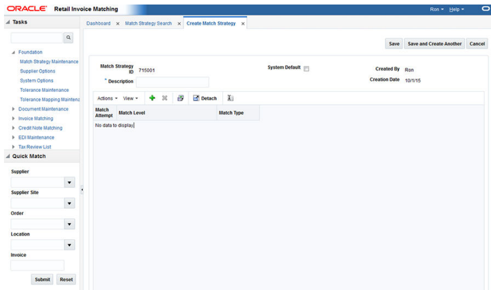
Figure 2-2 Create Match Strategy Window
