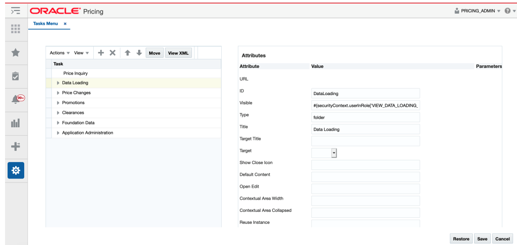
Figure 6-2 Table View
