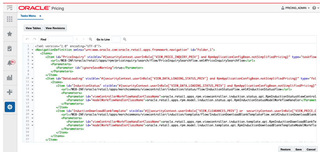
Figure 6-3 XML View
