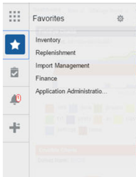
Figure 2-6 Favorites Area
