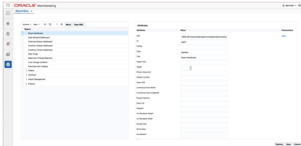
Figure 6-5 Table View
