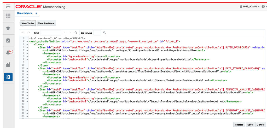
Figure 6-6 XML View
