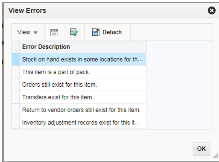
Figure 2-21 View Errors
