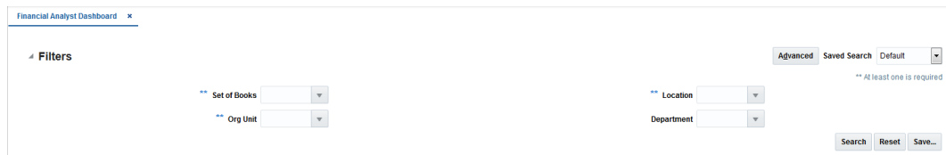
Figure 2-22 Filter Criteria
