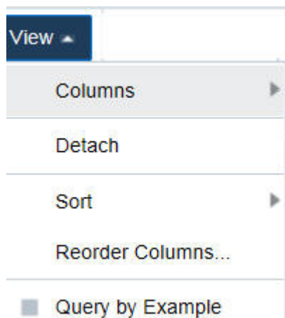
Figure 2-11 View Menu
