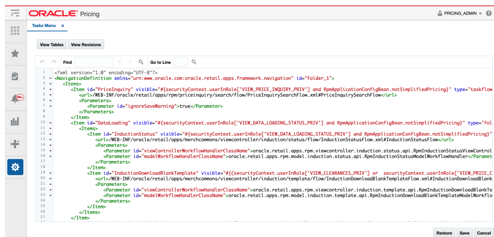
Figure 6-3 XML View
