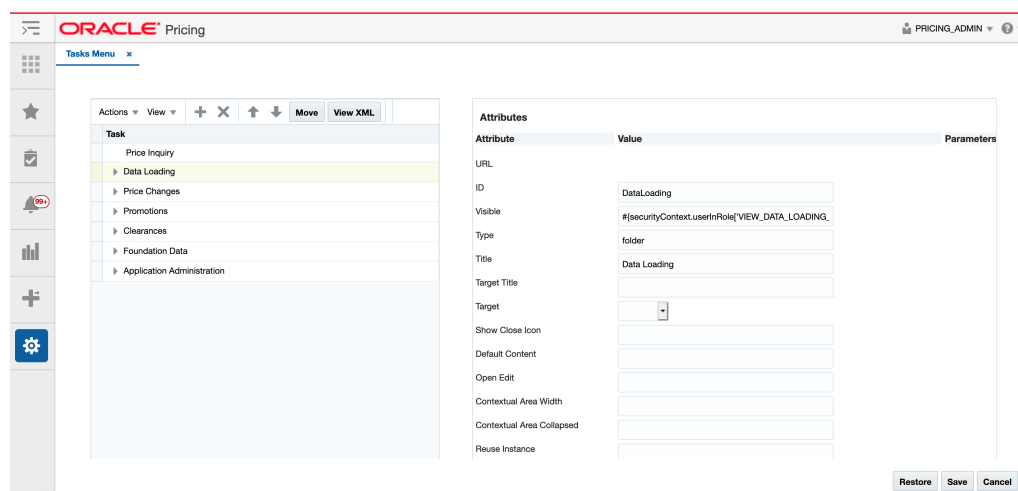
Figure 6-2 Table View
