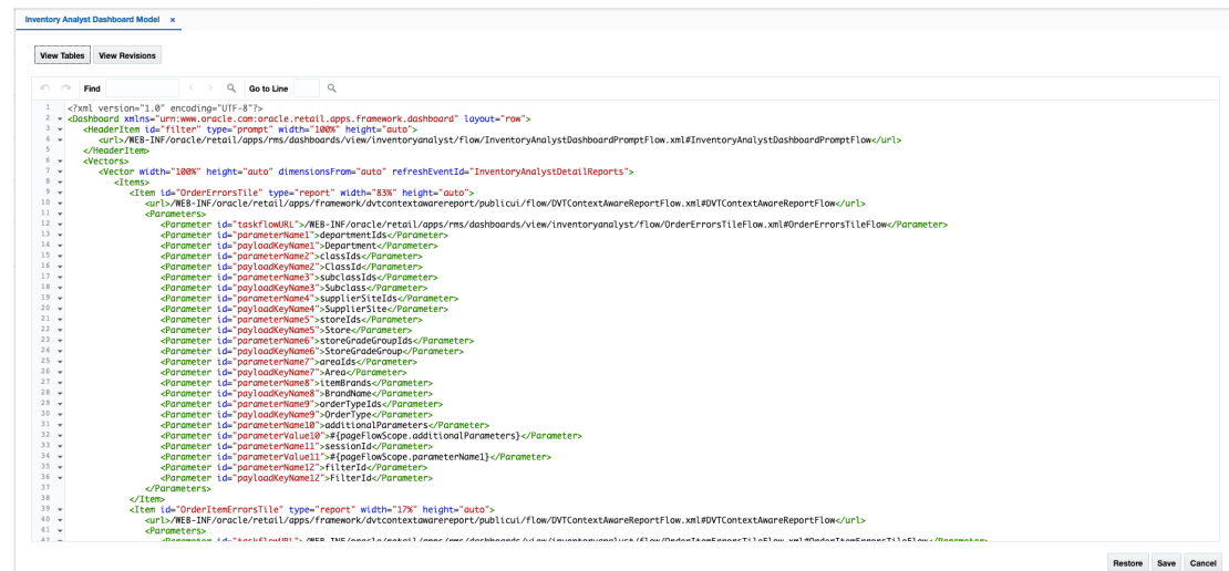
Figure 6-11 XML View
