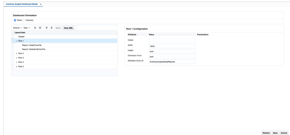
Figure 6-10 Table View
