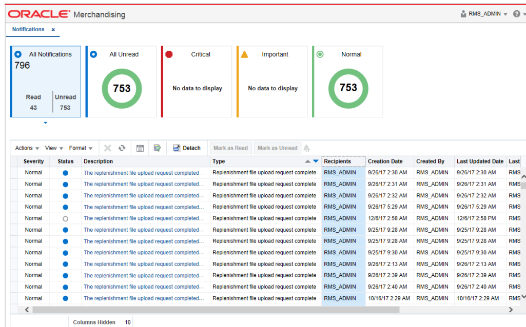
Figure 2-17 All Notifications
