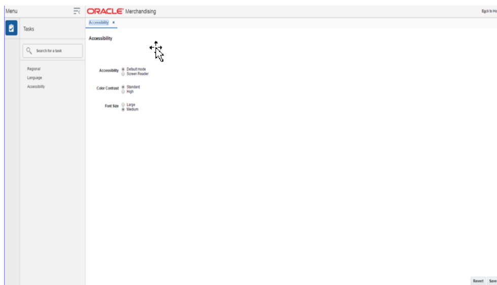
Figure 2-30 Accessibility Tab
