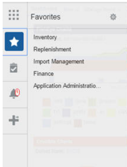
Figure 2-6 Favorites Area
