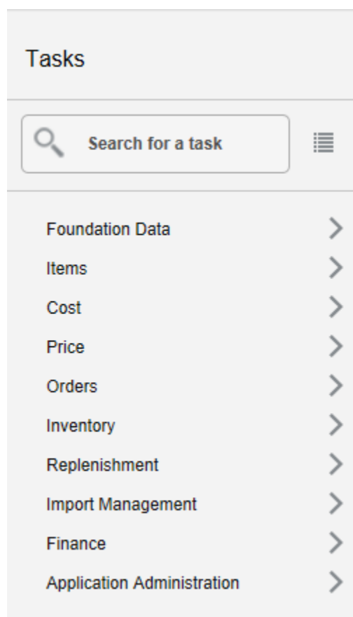
Figure 2-7 Tasks Menu
