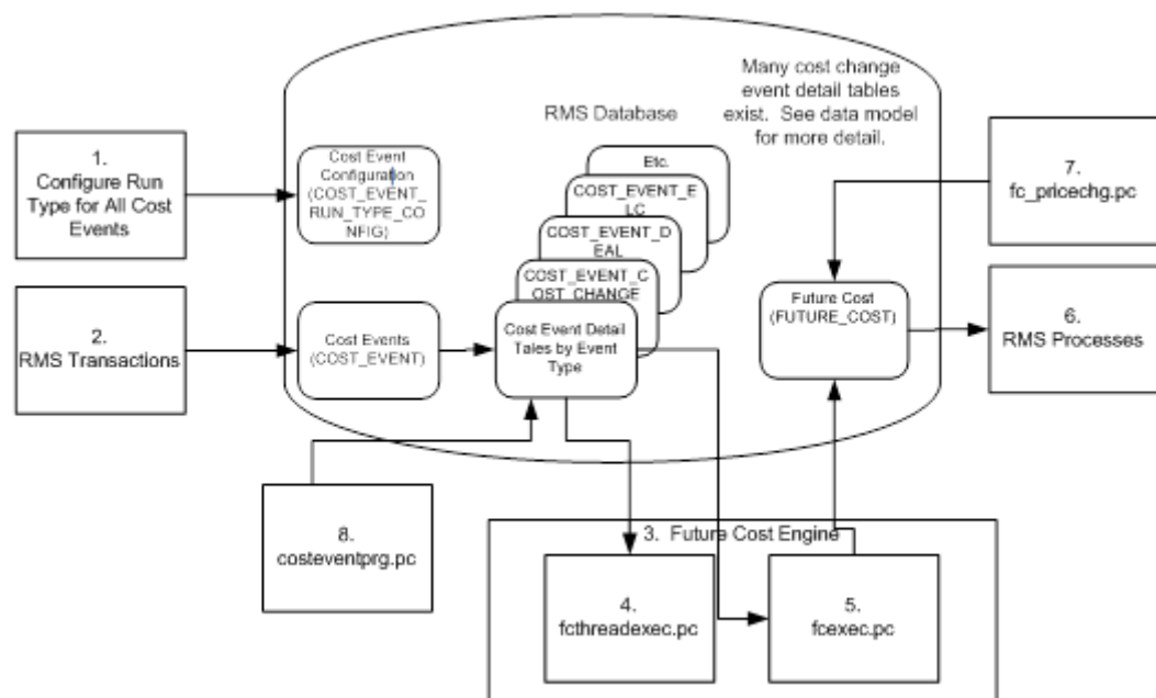
Figure 9-4 Future Cost Process
