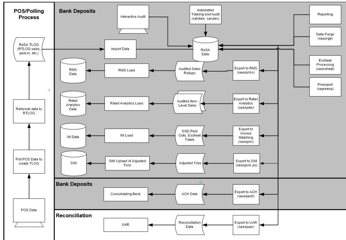
Figure 19-1 Oracle Retail Sales Audit Dataflow Diagram
