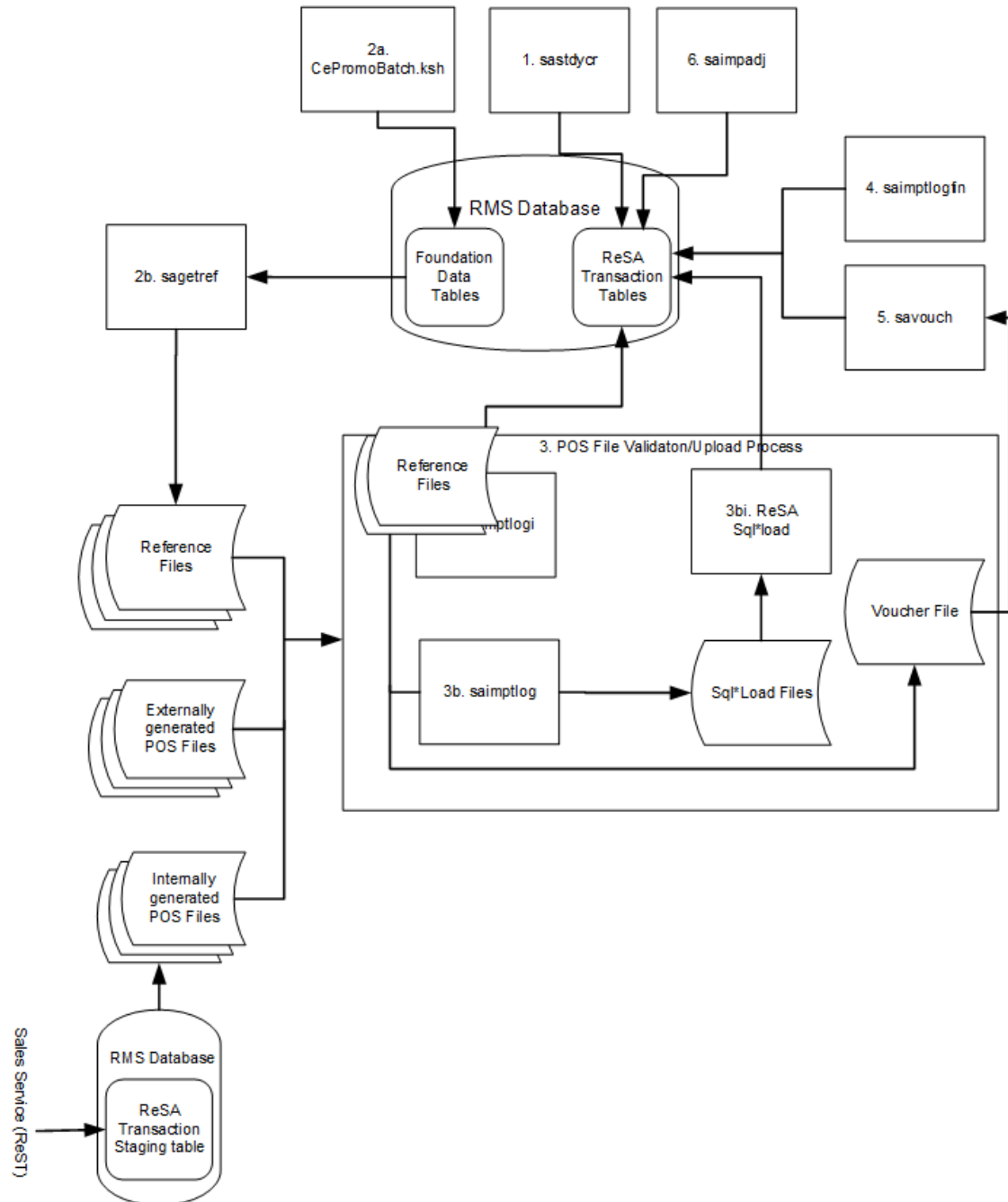
Figure 19-2 Oracle Retail Sales Import Process
