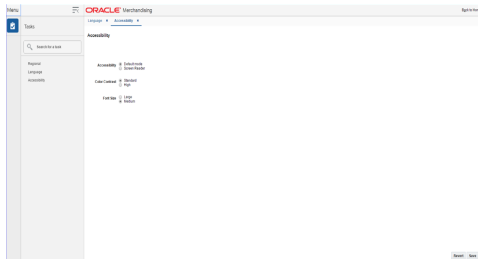
Figure 2-34 Accessibility Settings
