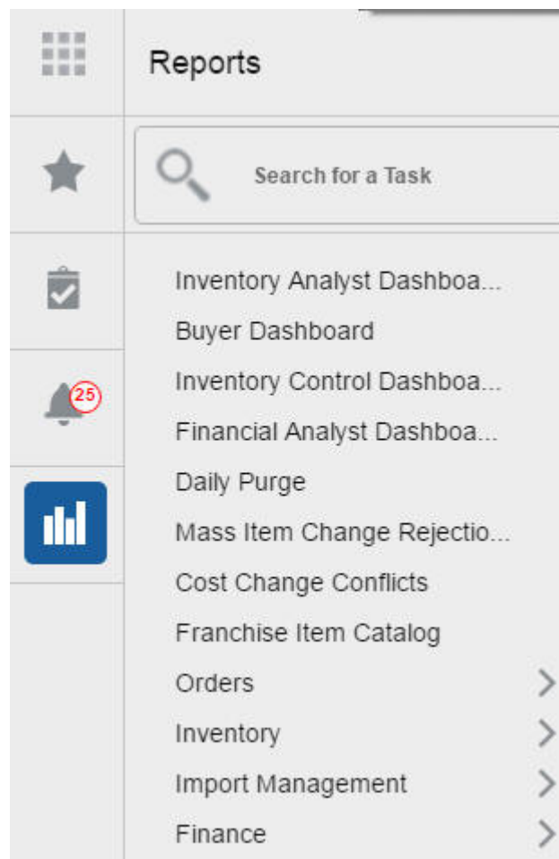
Figure 2-19 Reports Menu
