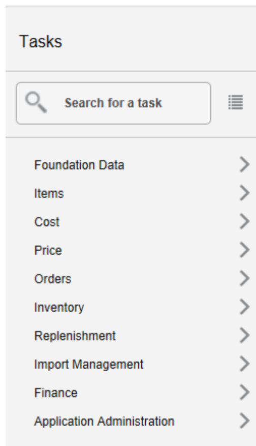
Figure 2-7 Tasks Menu
