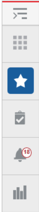
Figure 2-9 Notification Badge
