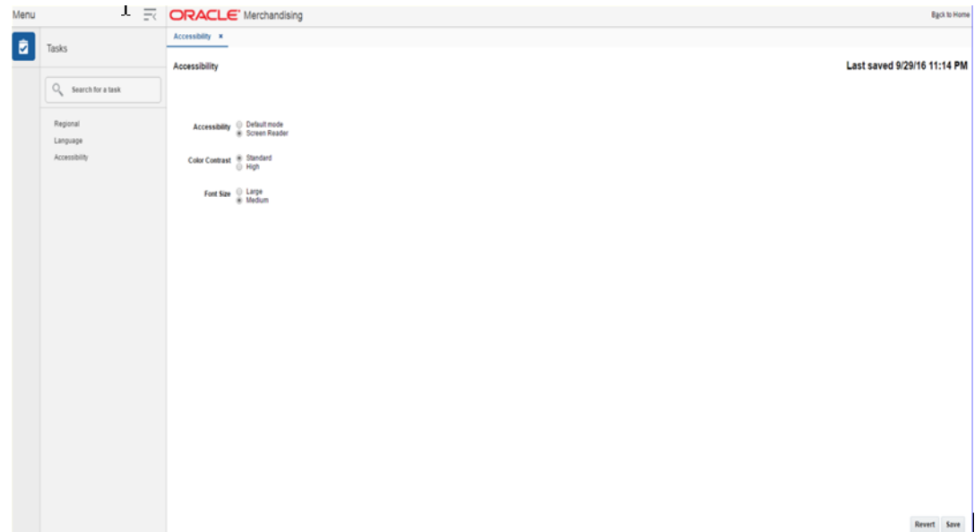
Figure 2-33 Accessibility Tab
