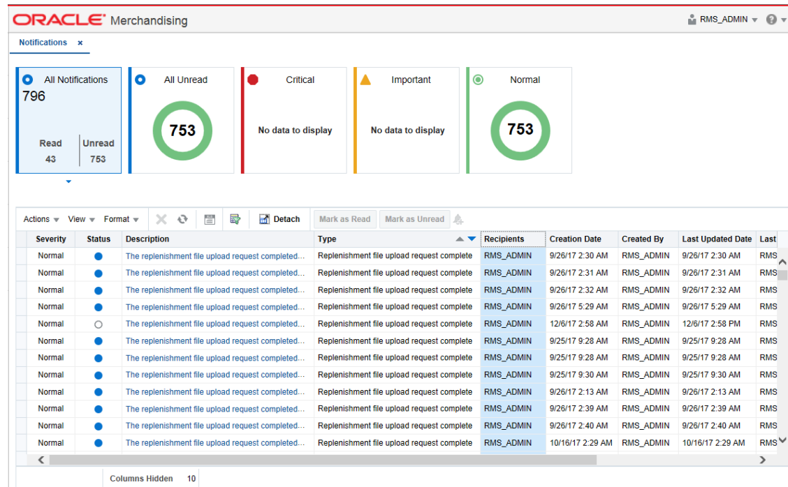
Figure 2-17 All Notifications
