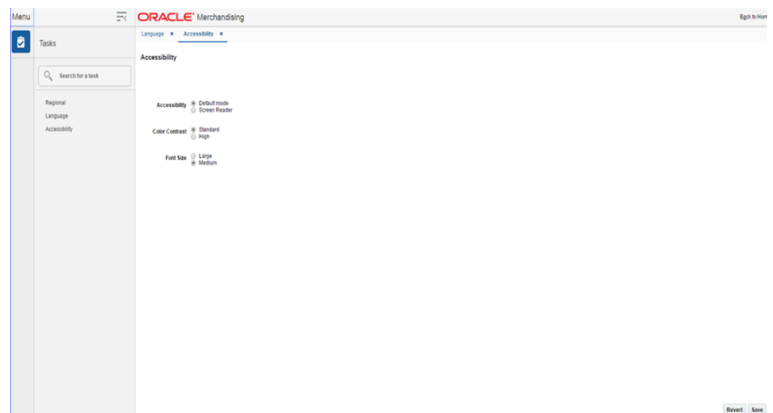
Figure 2-34 Accessibility Settings
