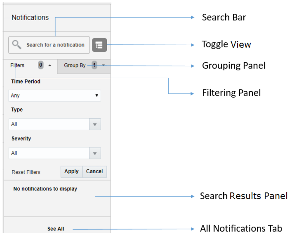
Figure 2-10 Notifications Sidebar
