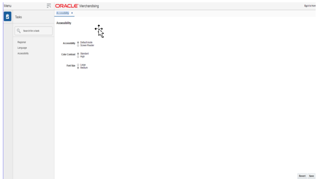
Figure 2-30 Accessibility Tab
