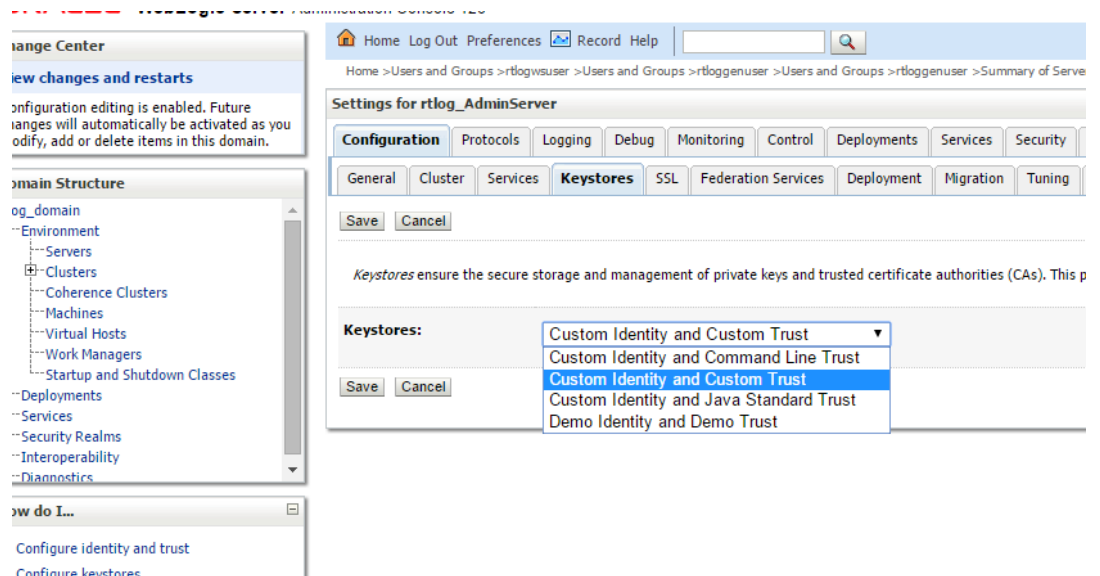
Figure 6-37 Keystores Settings
