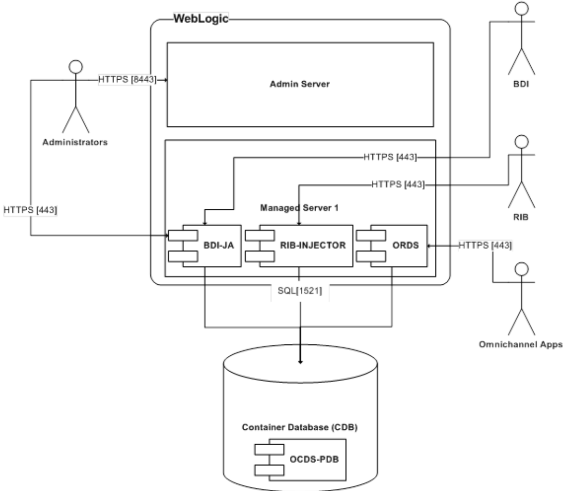
Figure 2-1 OCDS Component Diagram
