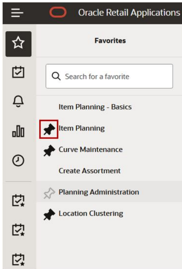
Figure 20-3 Pin Favorites
