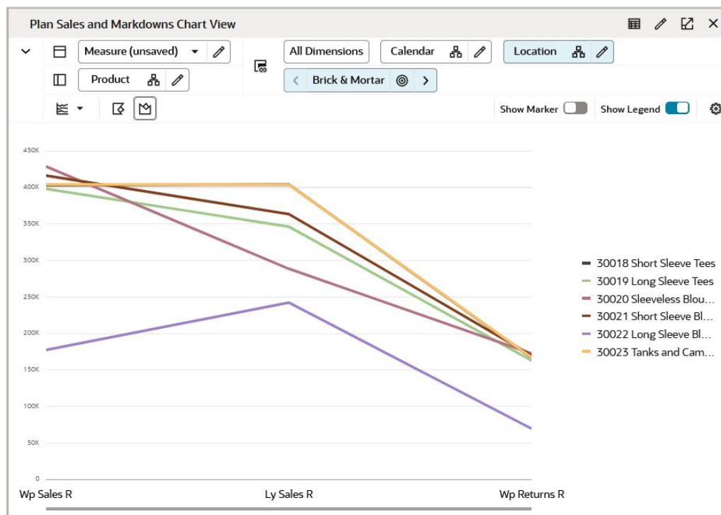
Figure 10-28 Line Chart
