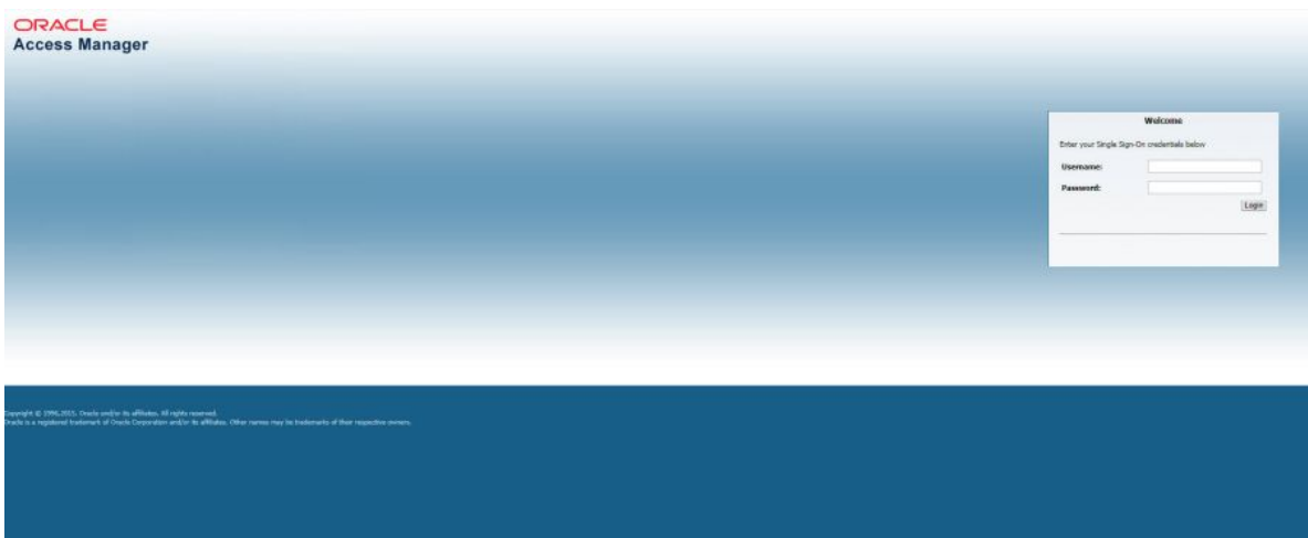
Figure 1-8 Login Window
