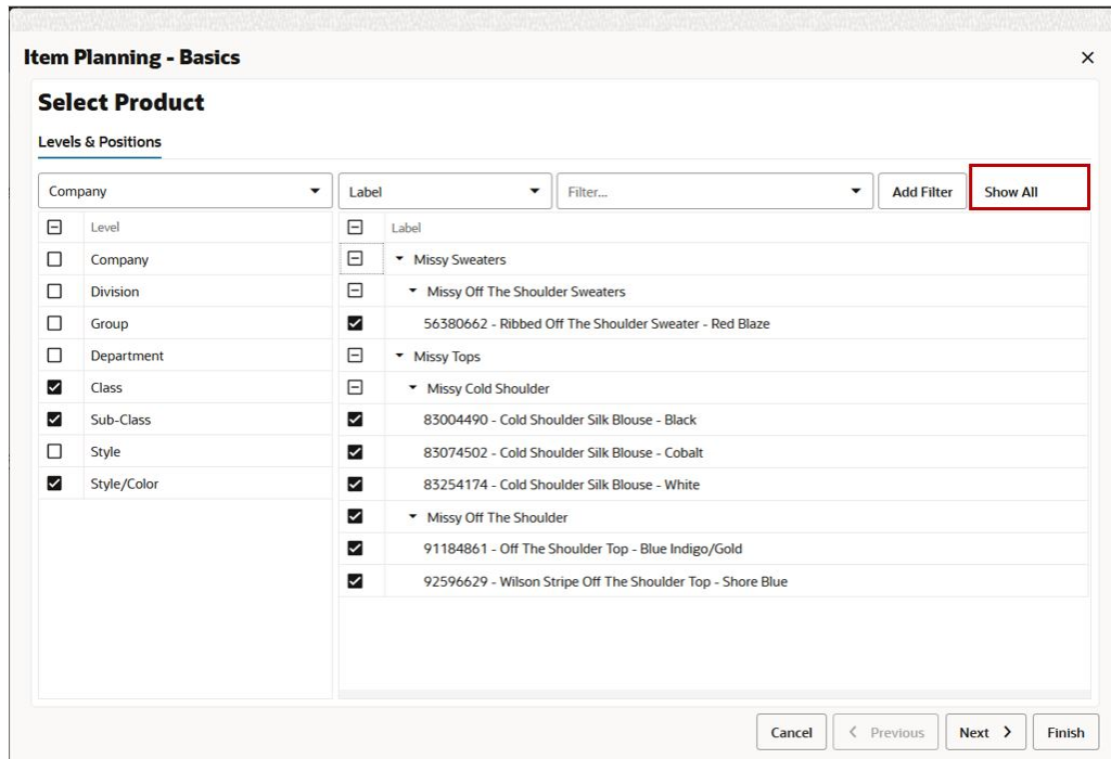
Figure 6-25 Show All
