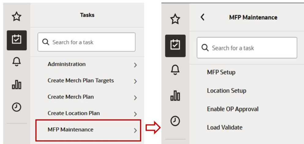
Figure 1-17 Taskflow
