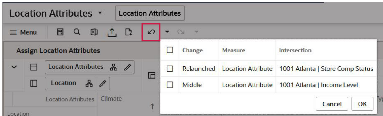
Figure 2-18 Undo Button
