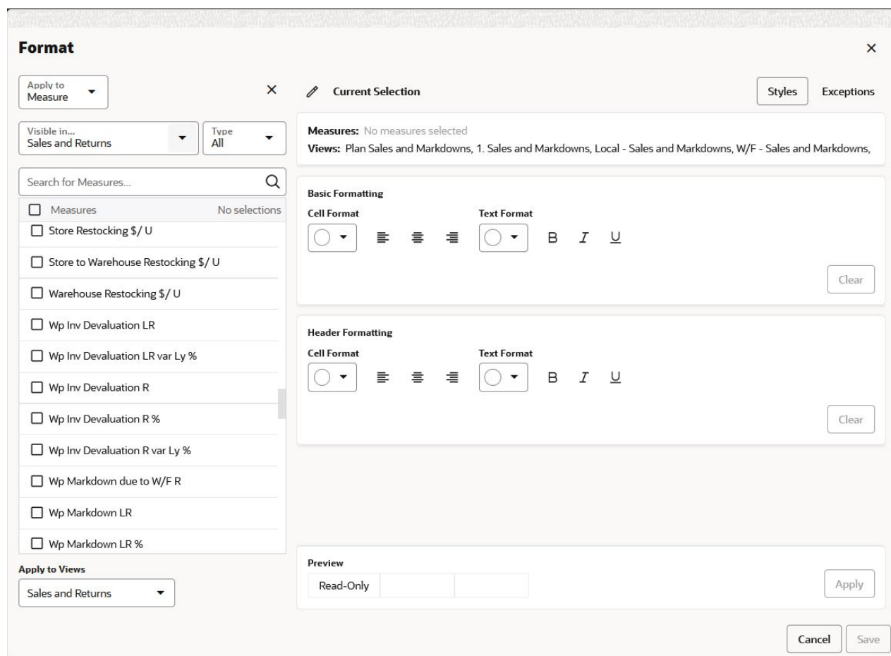
Figure 11-5 Styles Tab
