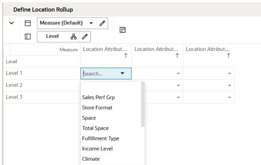
Figure 1-1 Dynamic Hierarchy
