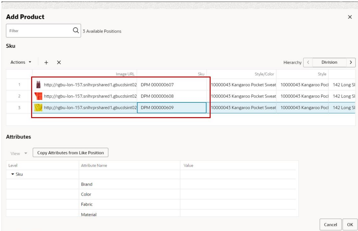
Figure 14-5 Add Product
