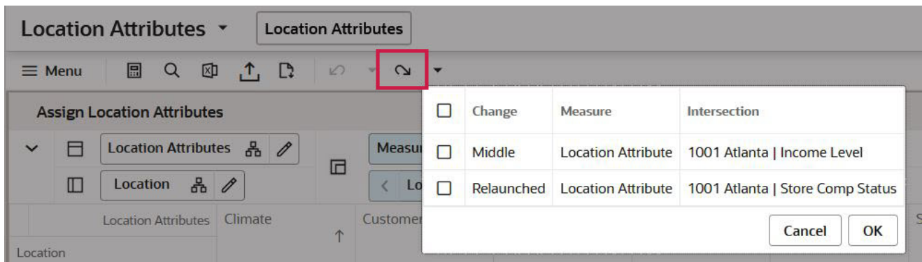
Figure 2-19 Redo
