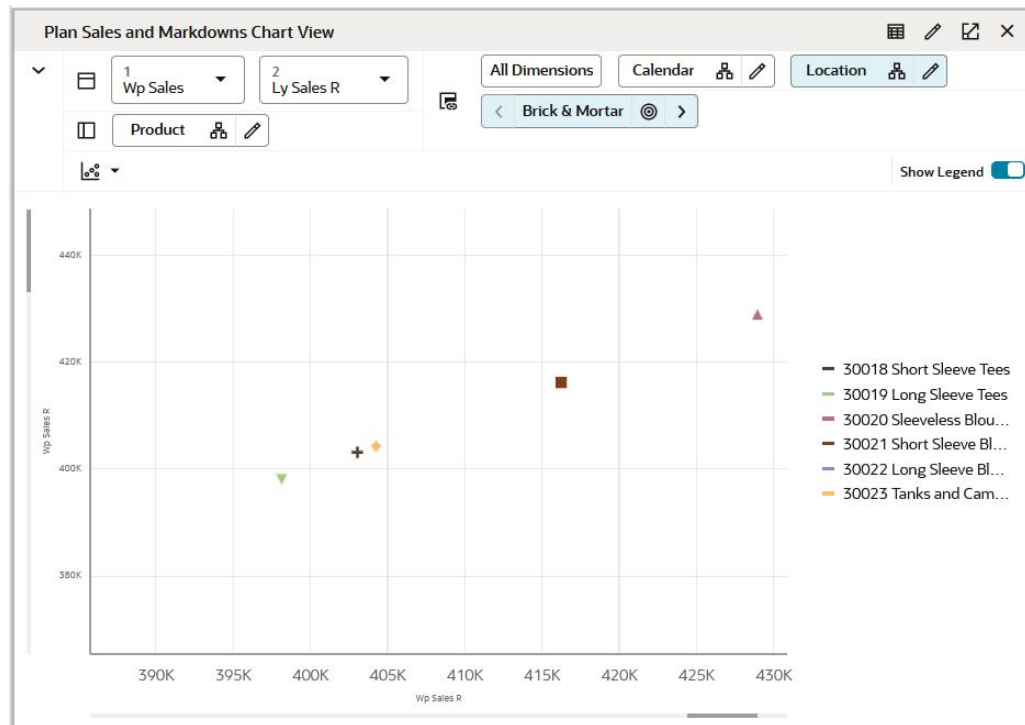
Figure 10-32 Scatter Chart
