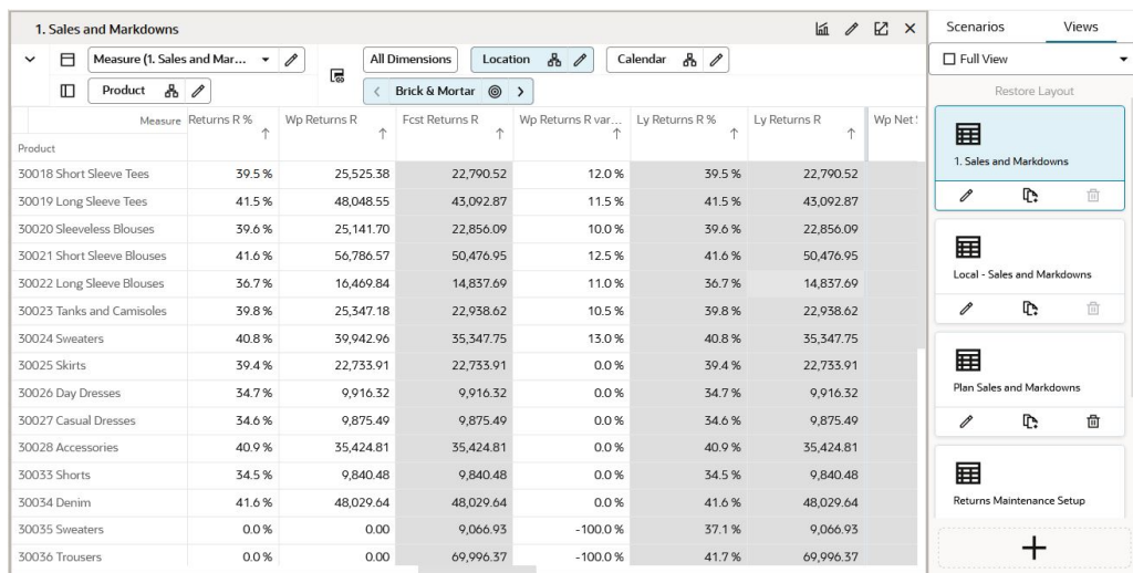
Figure 9-16 View List
