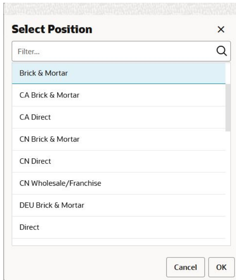
Figure 2-31 Select Position
