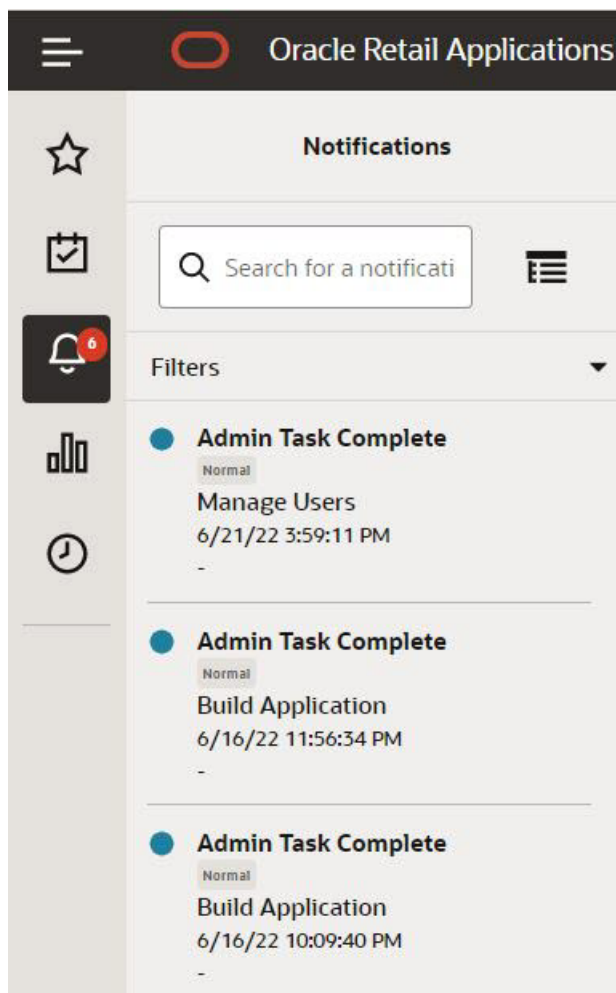
Figure 2-4 Using Notifications
