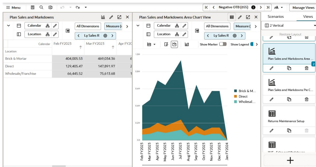
Figure 10-25 Multi-group Chart
