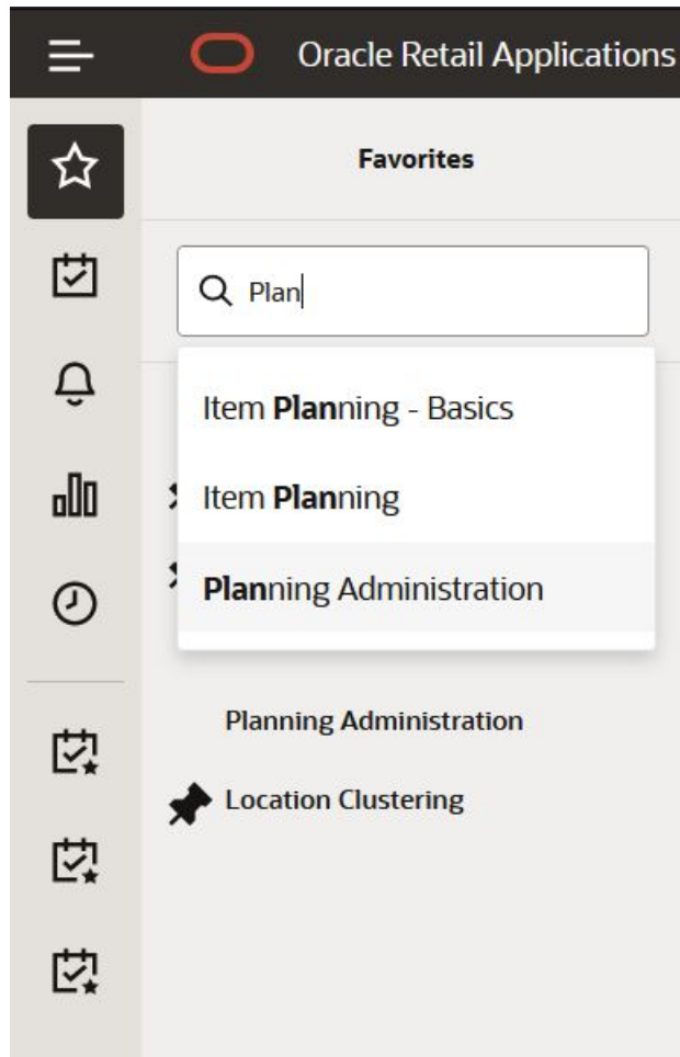
Figure 20-5 Search Favorites
