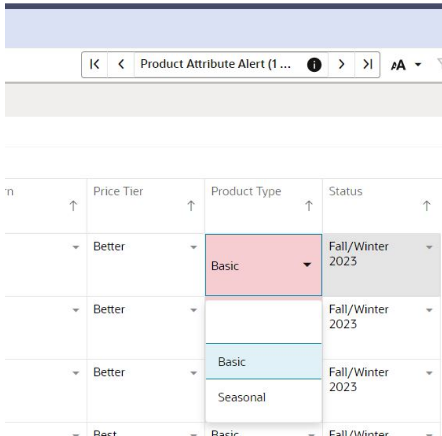
Figure 15-10 Resolving Alerts
