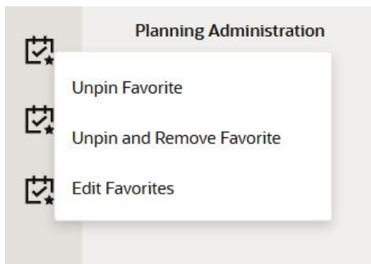
Figure 20-4 Unpin Favorite
