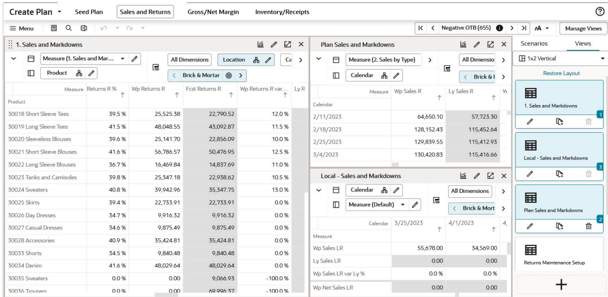
Figure 9-15 Restore Layout
