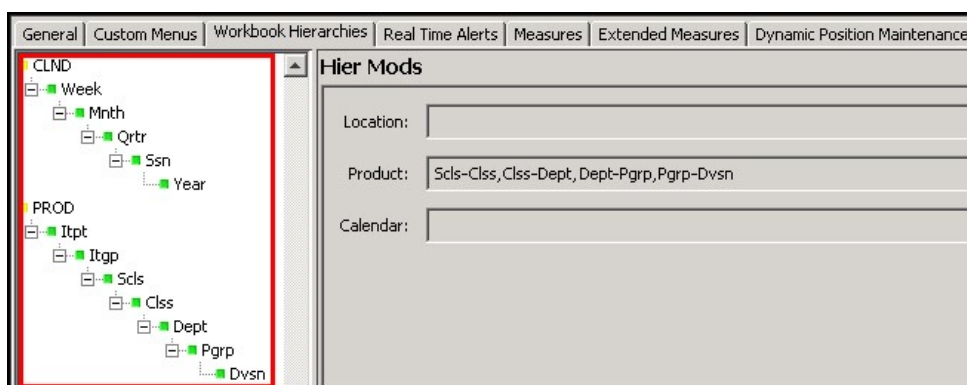
Figure 4-103 Displayed Hierarchies and Dimensions in the Workbook Hierarchies Tab
