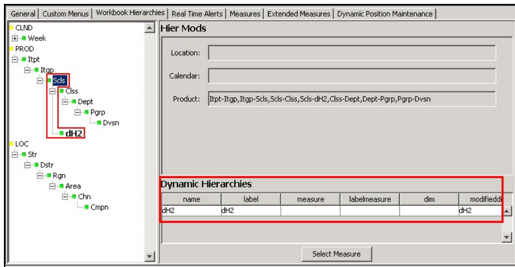
Figure 4-117 New Workbook Dimension
