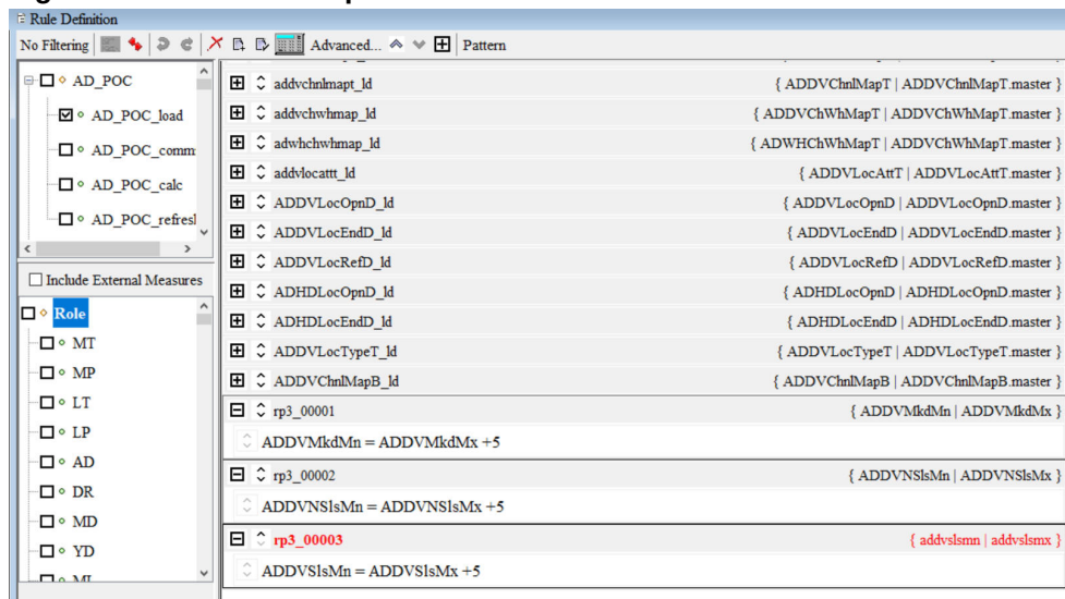
Figure 4-71 New and Updated Rules
