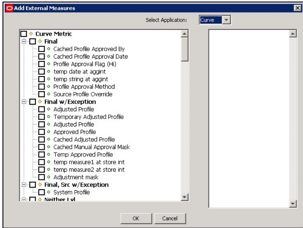
Figure 4-23 Add External Measures Window
