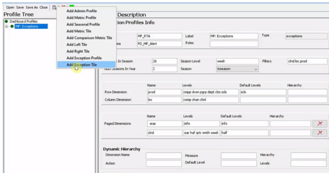
Figure 12-31 Adding an Exception Tile
