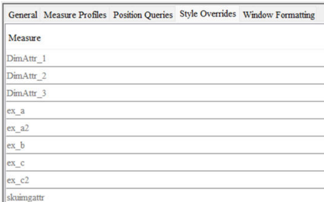
Figure 4-169 Style Override Panel for a Tiled View Worksheet Showing a Tile Measure
