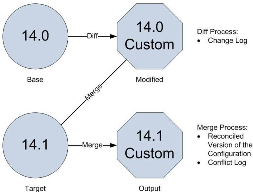
Figure D-1 The Diff and Merge Processes
