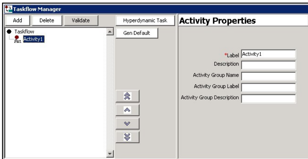
Figure 3-47 Activity1 in the Taskflow
