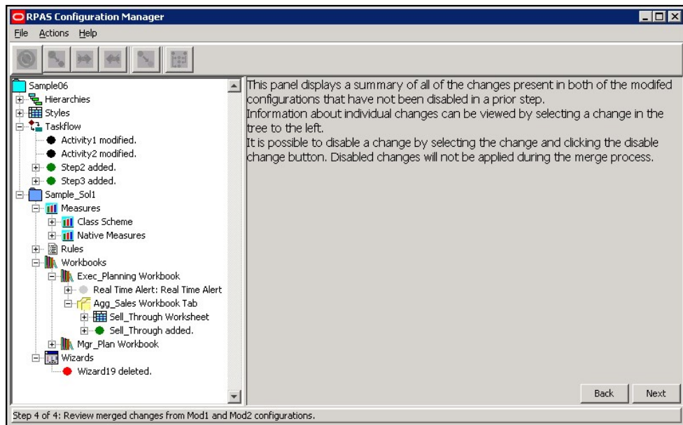
Figure D-8 Merged Changes Review
