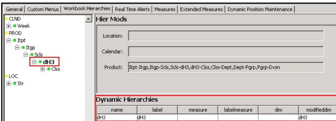
Figure 4-119 New Workbook-Only Dimension
