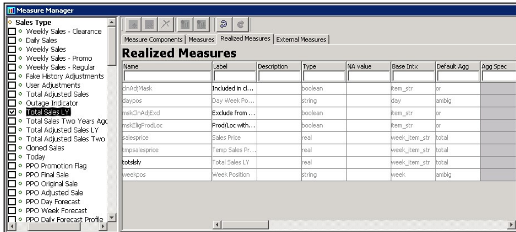
Figure 4-20 Measure Manager Realized Measures Tab
