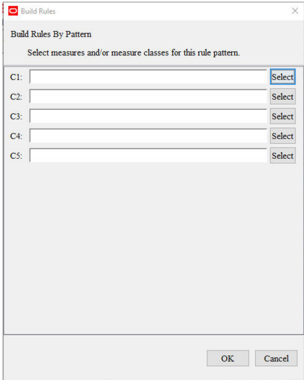
Figure 4-66 Build Rules Dialog Box
