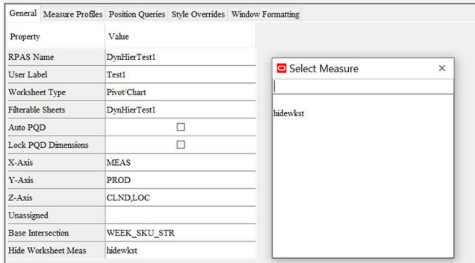
Figure 4-161 Select a Hide Worksheet Measure
