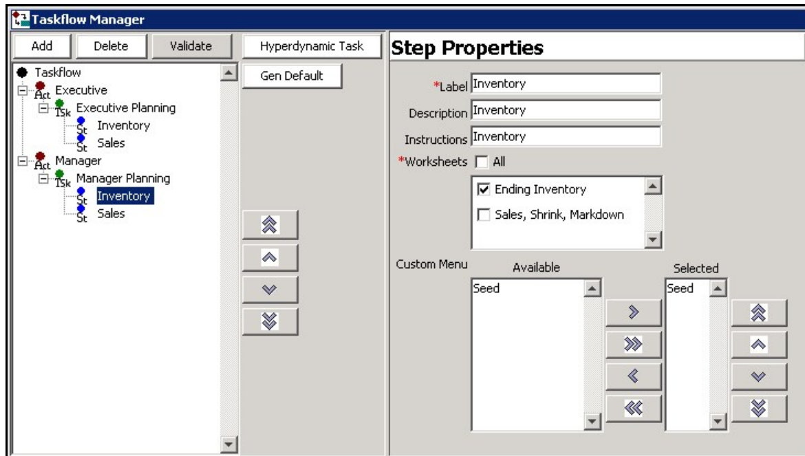
Figure 3-53 Step Properties
