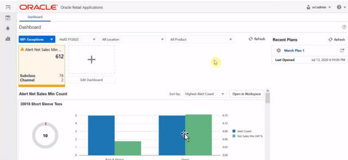
Figure 12-33 Dashboard Instance
