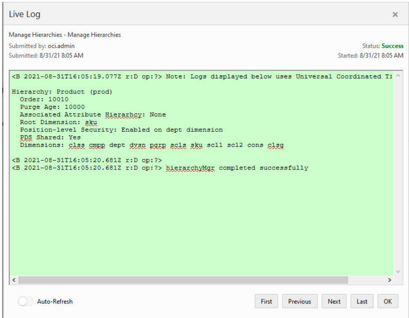
Figure 5-45 Sample Live Log Output for Manage Hierarchies Task
