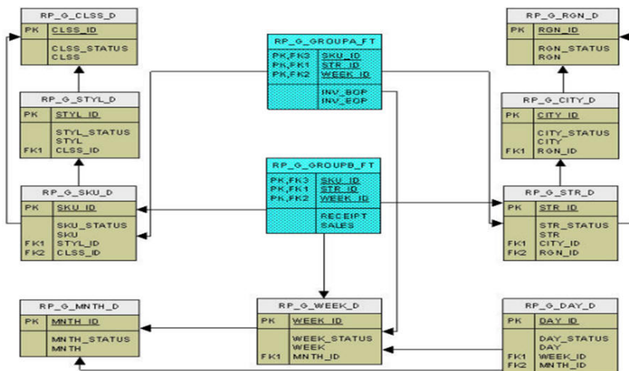
Figure 3-2 PDS Entity Relationship Diagram
