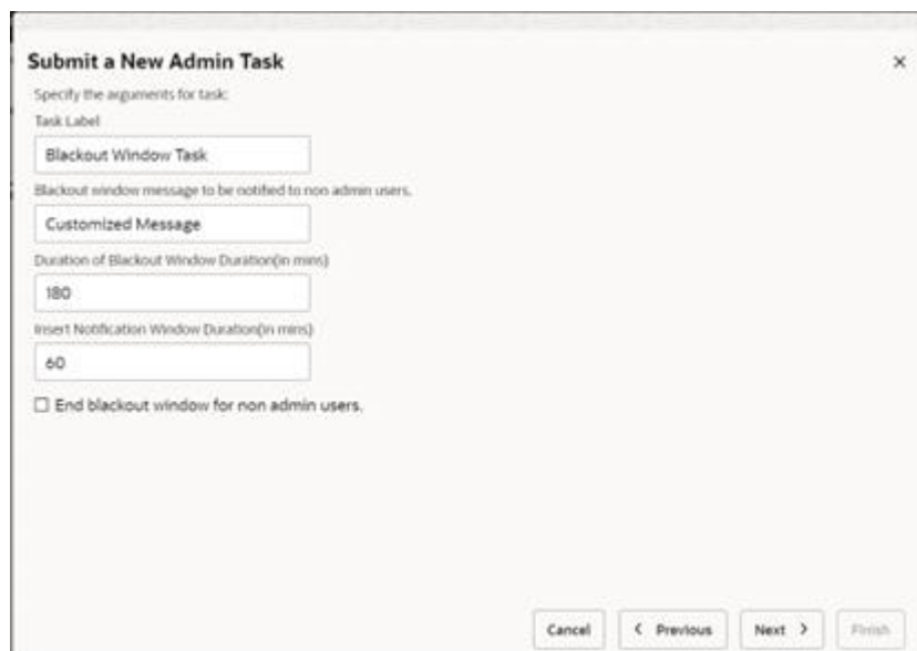
Figure 19-2 Blackout Window Arguments
