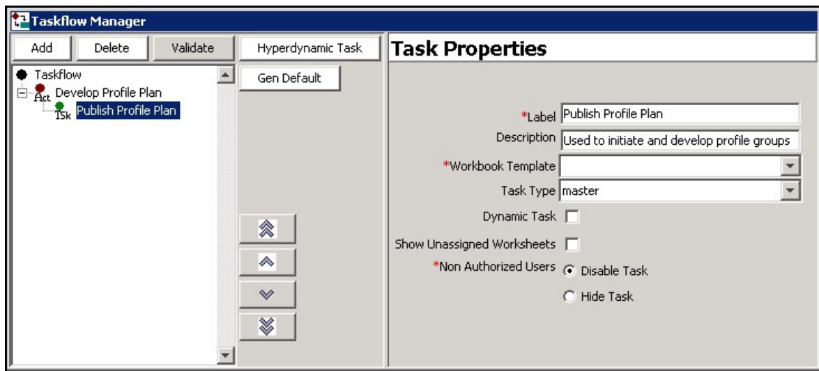
Figure 3-51 Task Properties
