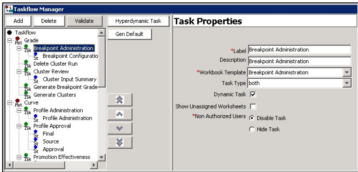
Figure 3-48 Activity Properties
