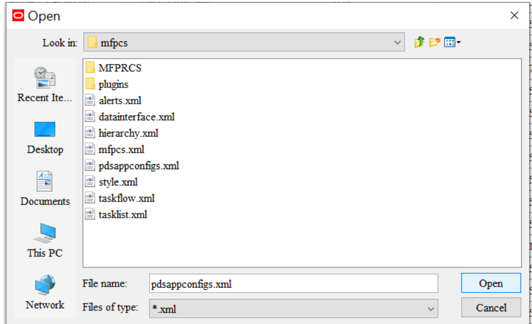
Figure 11-17 Load pdsappconfig.xml
