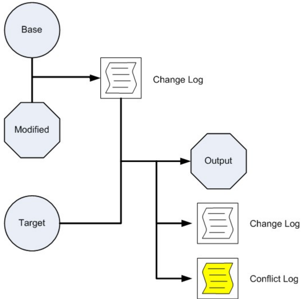
Figure D-4 diffAndMerge Process
