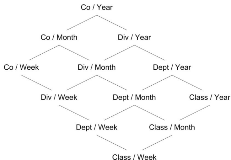
Figure A-1 Hierarchical Protection Processing Parent-Child Relationships
