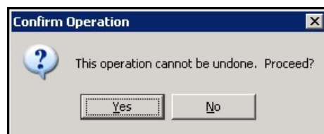
Figure 4-53 Confirm Operations
