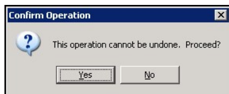
Figure 4-55 Confirm Operation
