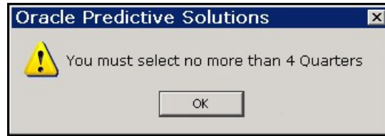
Figure 4-78 Error Message
