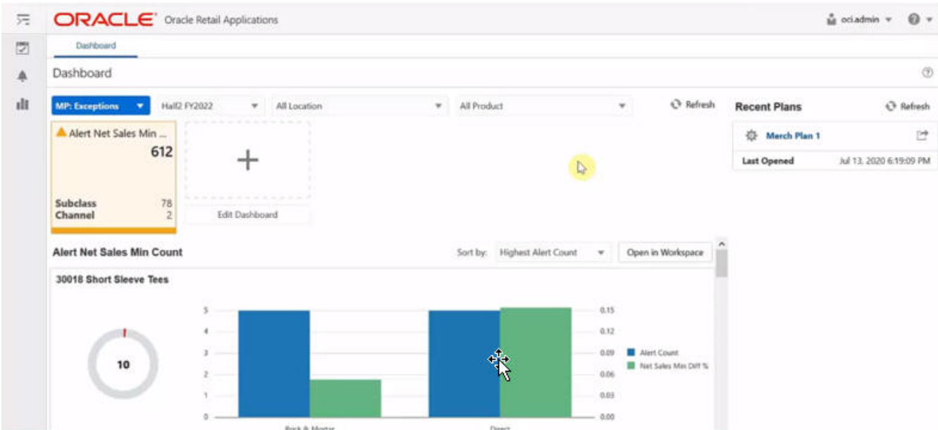
Figure 12-33 Dashboard Instance
