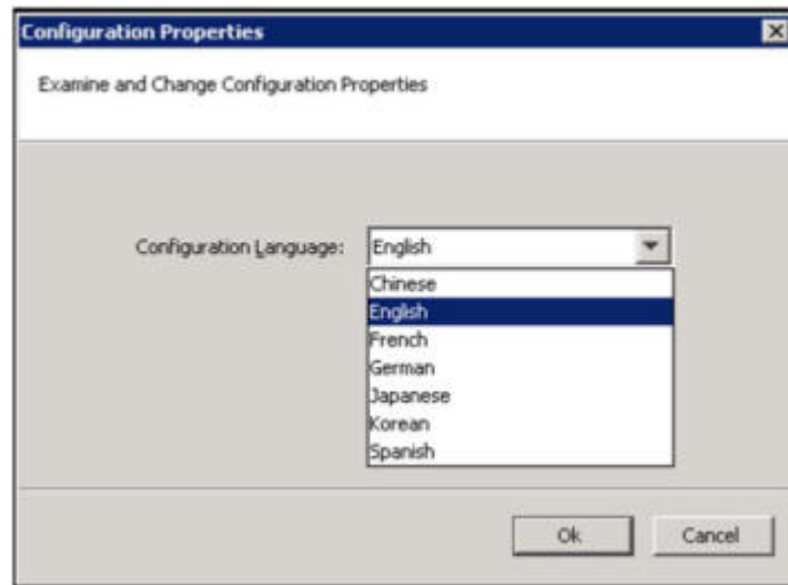
Figure 11-20 Configuration Properties
