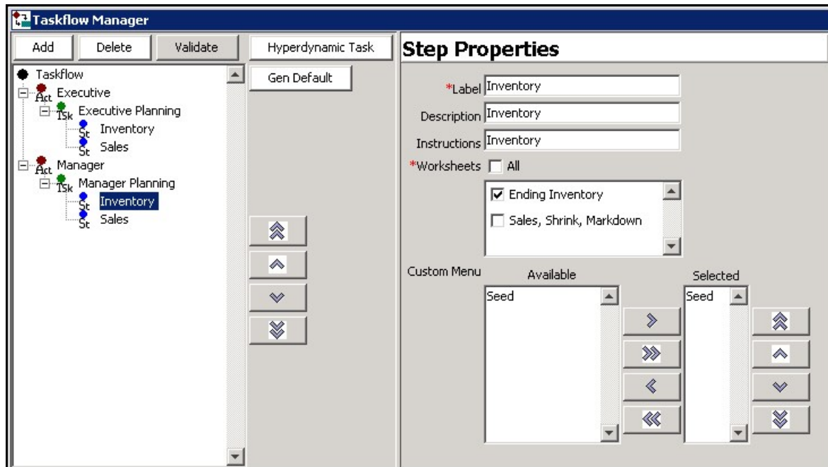
Figure 3-53 Step Properties
