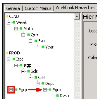
Figure 4-108 Restored Dimension
