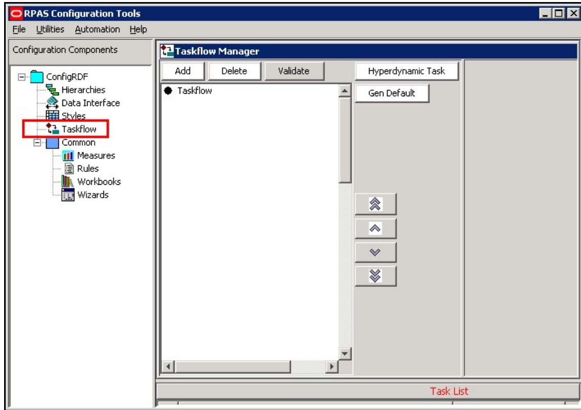
Figure 3-45 Taskflow Manager
