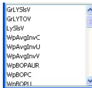
Figure 4-40 Measure Names
