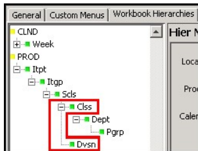
Figure 4-111 New Rollup
