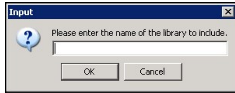
Figure 9-3 Input Window
