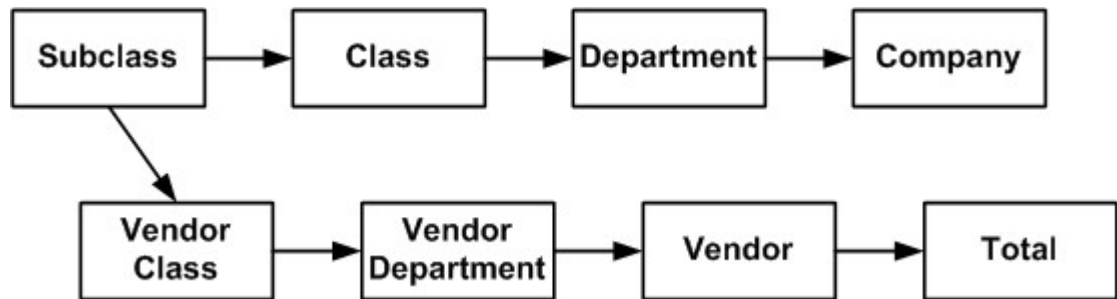
Figure 4-101 Workbook Dimensions
