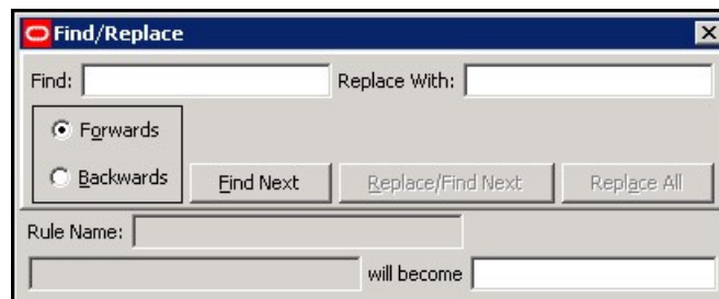
Figure 4-58 Find/Replace Window
