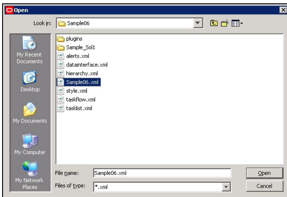
Figure 3-3 Open Window
