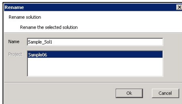
Figure 4-3 Rename Window
