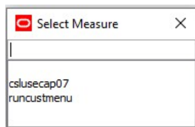
Figure 4-96 Select Measure
