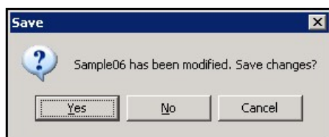
Figure 3-8 Save Window
