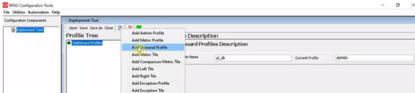
Figure 12-18 Seasonal Profile
