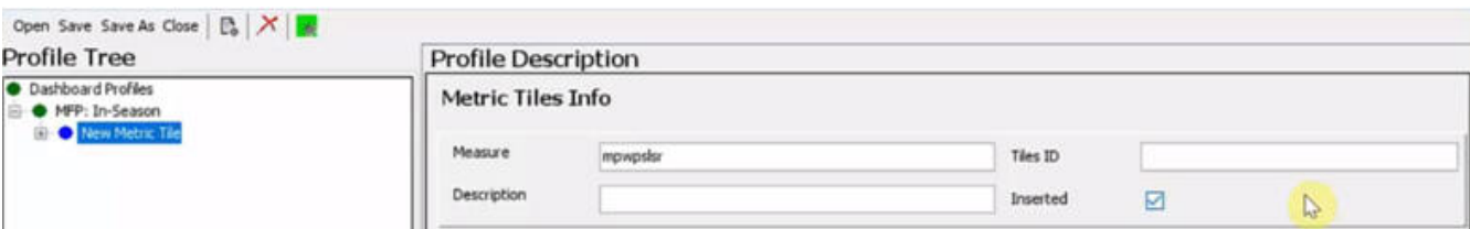
Figure 12-23 Measure Name
