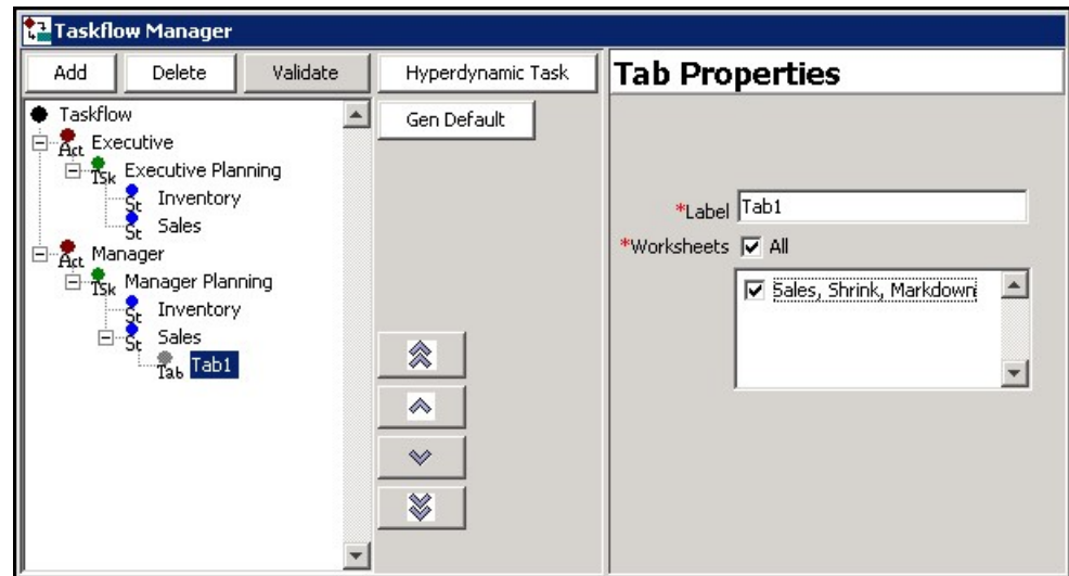
Figure 3-55 Tab Properties
