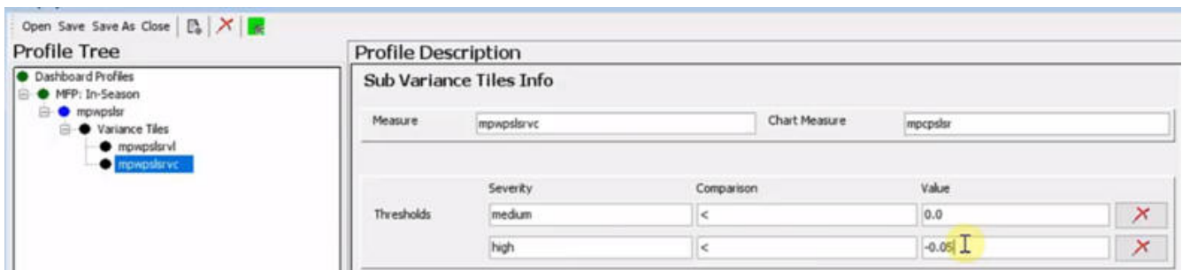
Figure 12-28 Flag Errors
