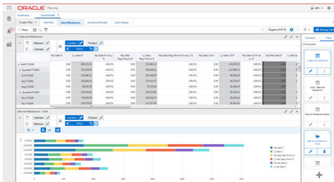
Figure 7-3 MFPRCS Workspace
