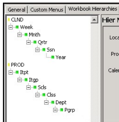
Figure 4-105 Removed Dimension
