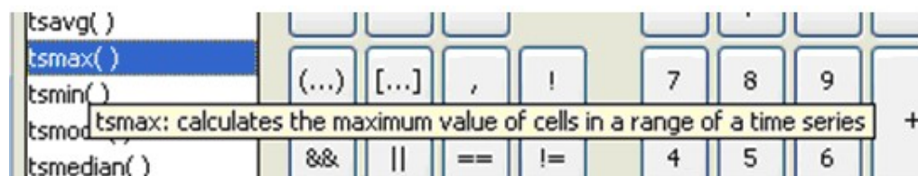
Figure 4-41 Tooltip
