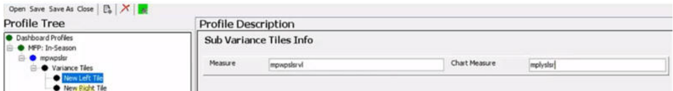
Figure 12-25 Compare Sales
