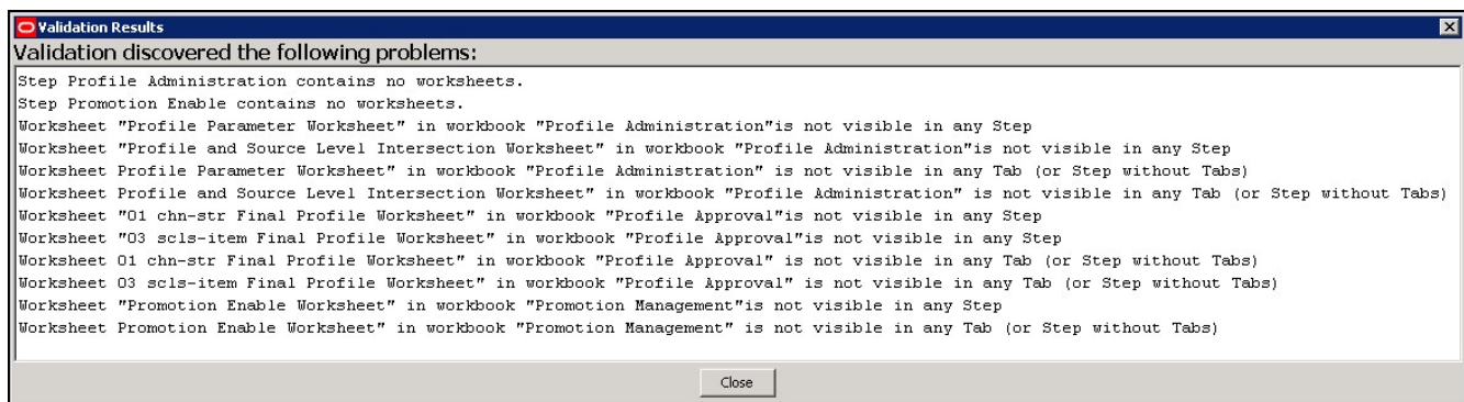
Figure 3-58 Validation Results
