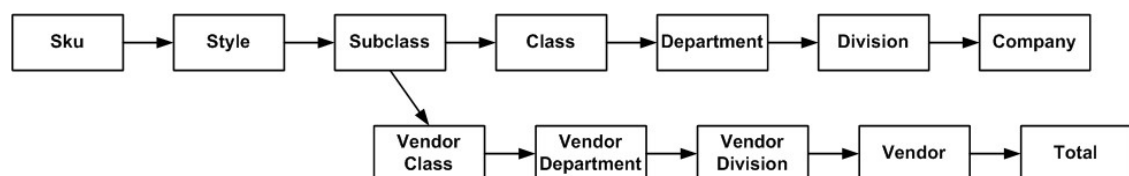
Figure 4-100 Product Hierarchy
