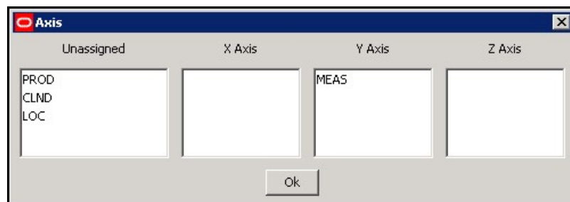
Figure 4-76 Axis Window
