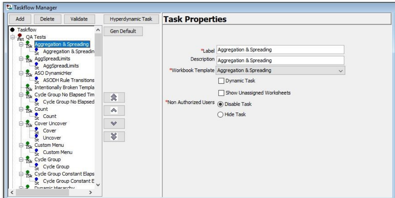
Figure 3-50 Task Properties
