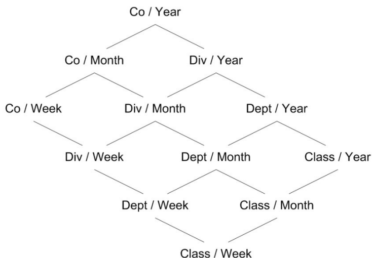
Figure A-1 Hierarchical Protection Processing Parent-Child Relationships
