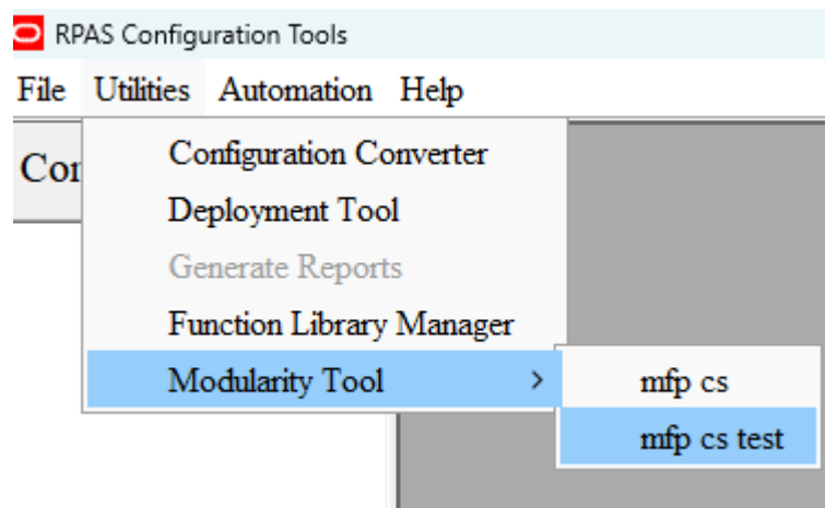
Figure 9-5 Modularity Tool SubMenu for Application Selection
