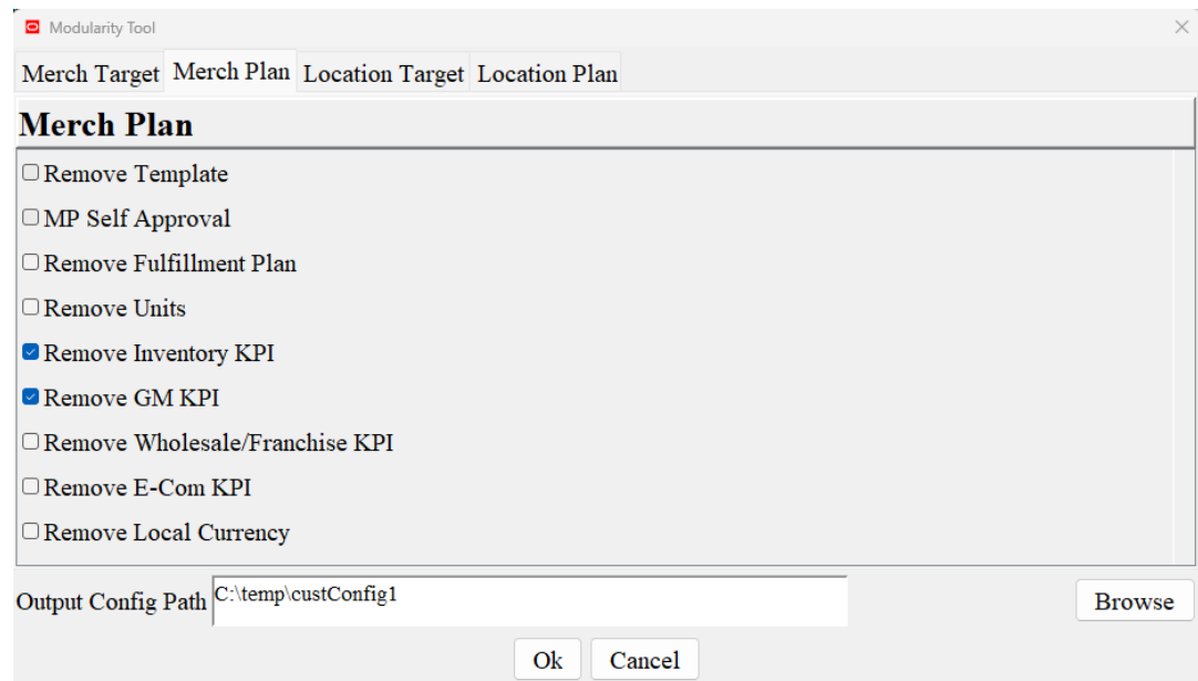
Figure 9-7 Specify Full Path to the Parent Directory of the Output Configuration
