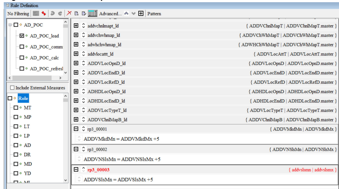
Figure 4-71 New and Updated Rules
