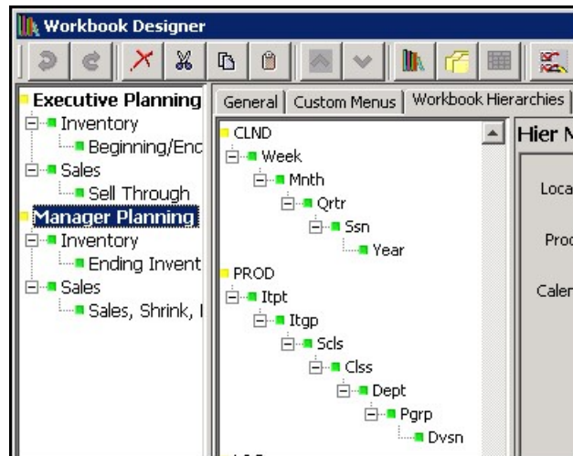
Figure 4-102 Workbook List in Workbook Designer
