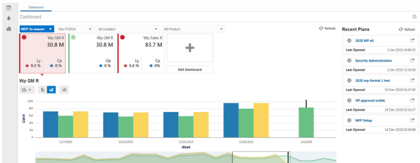
Figure 2-1 Dashboard Window
