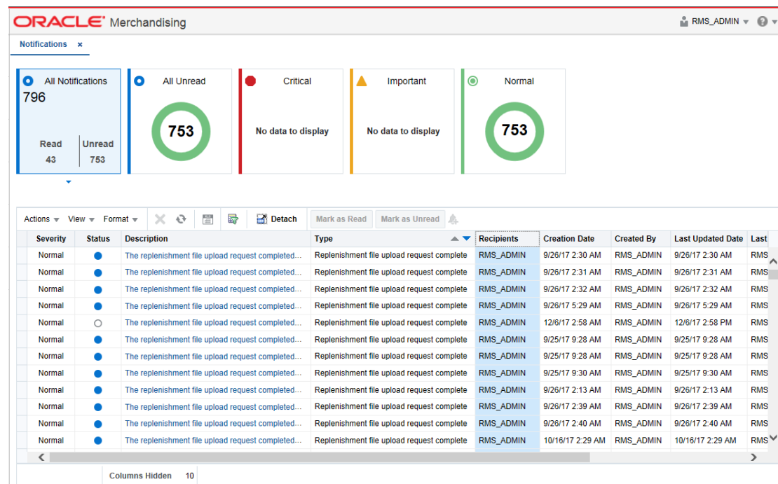
Figure 7-9 All Notifications
