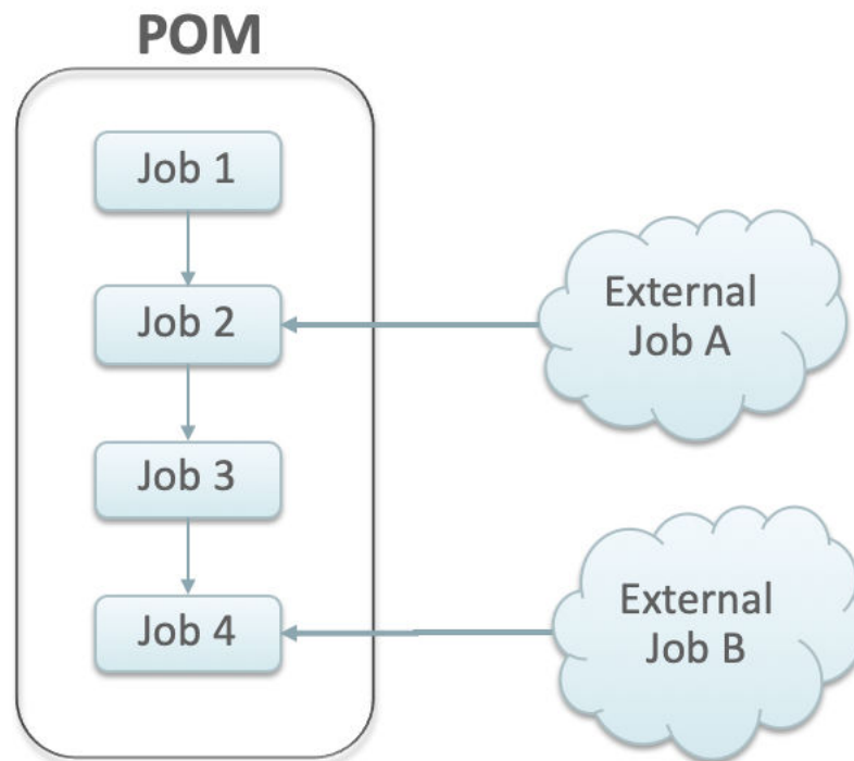
Figure 3-6 External Dependency
