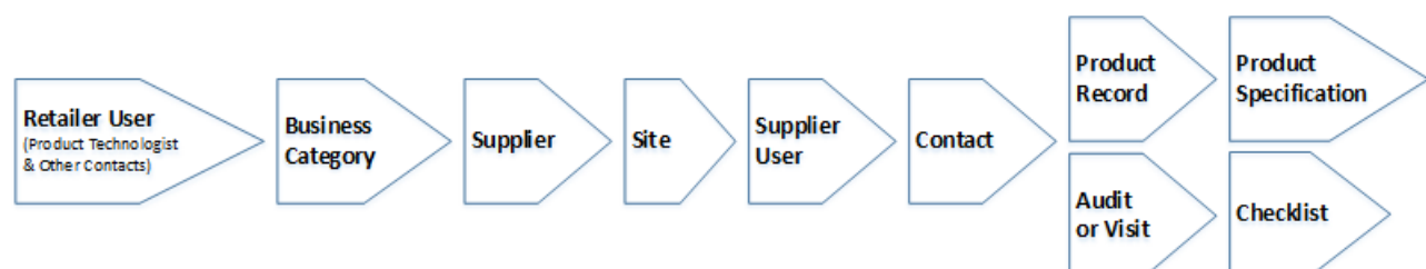
Figure 3-1 Dependencies
