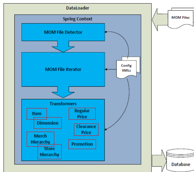
Figure 2–4 DataLoader Flow
