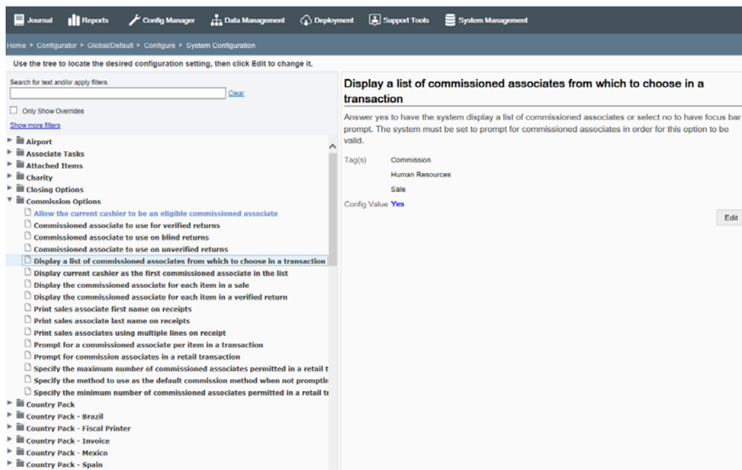
Figure 5-37 System Configuration Page - Configuration Option Detail
