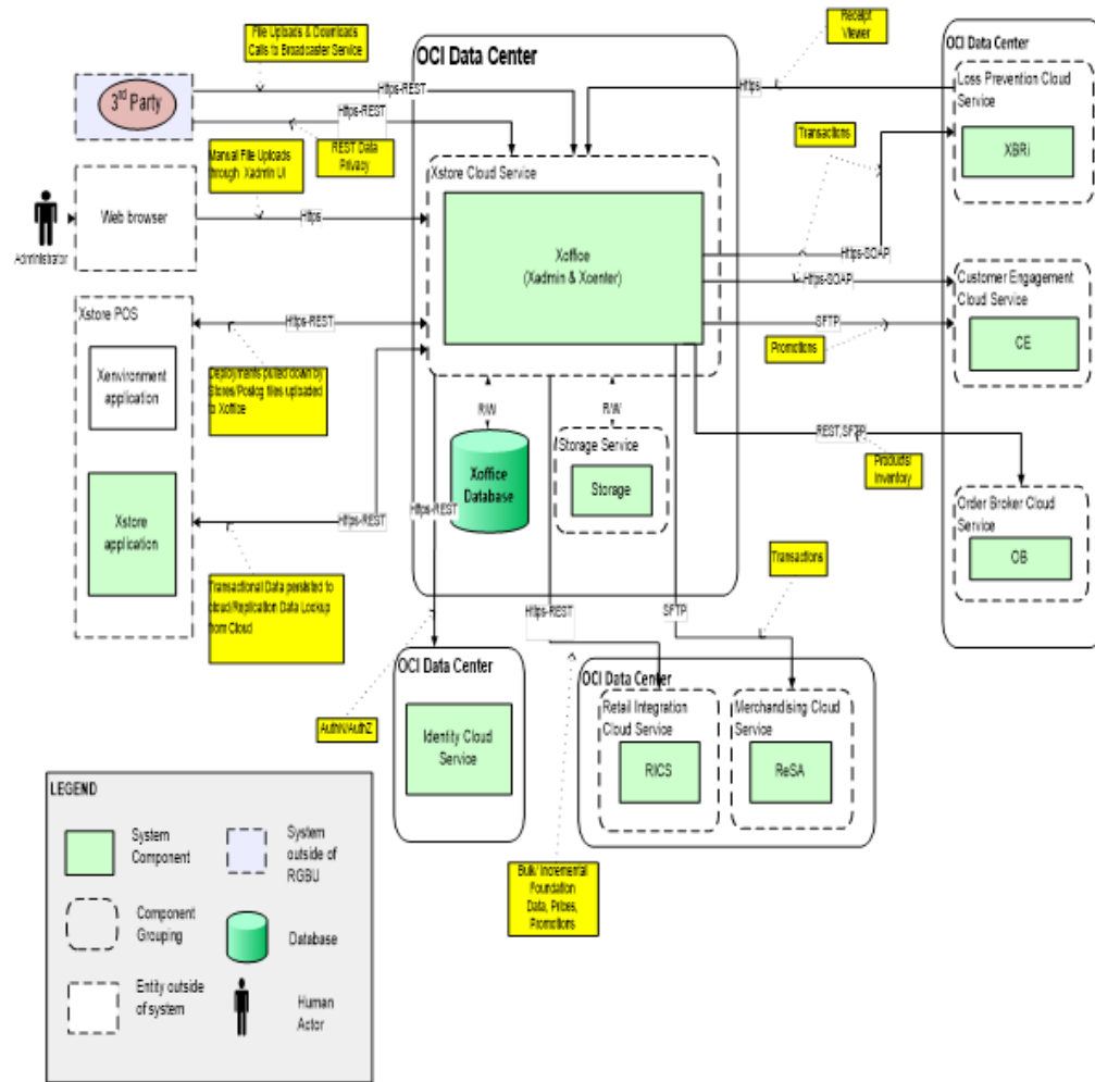
Figure 3-1 Xstore Office Cloud Service Integration Data Flow
