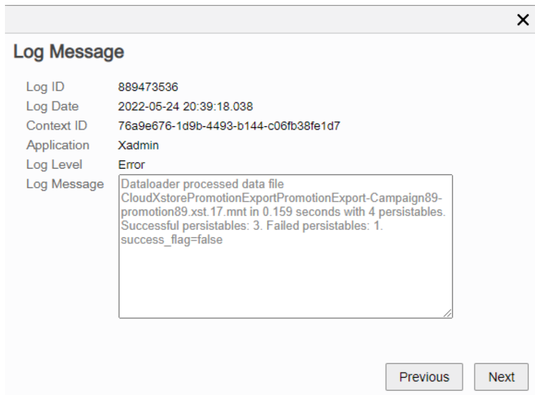
Figure 3-7 Log Message
