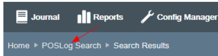
Figure 10-18 POSLog Breadcrumb
