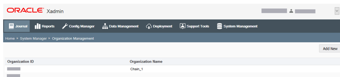
Figure 3-2 Organization Management
