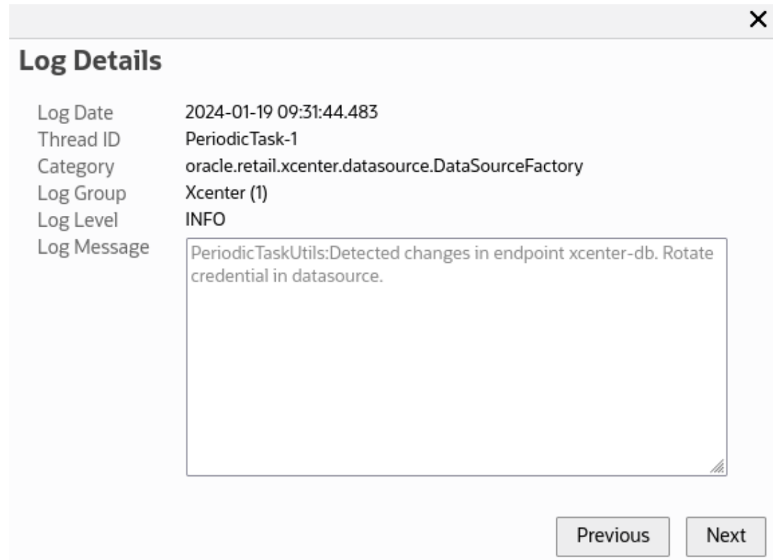
Figure 3-7 Log Details
