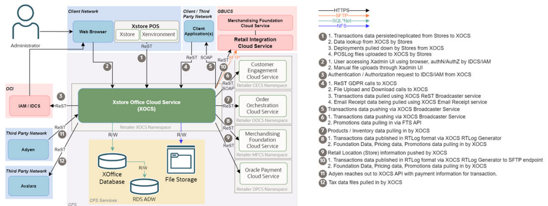
Figure 1-1 Architecture Model
