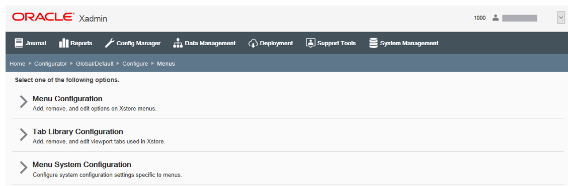
Figure 5-10 Menu Options
