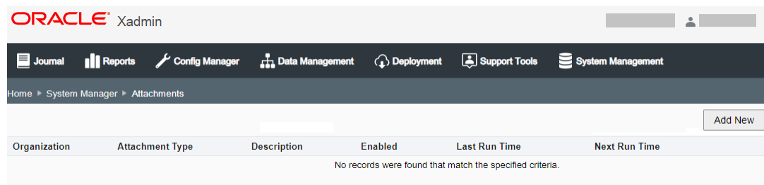
Figure 3-8 Attachments Page
