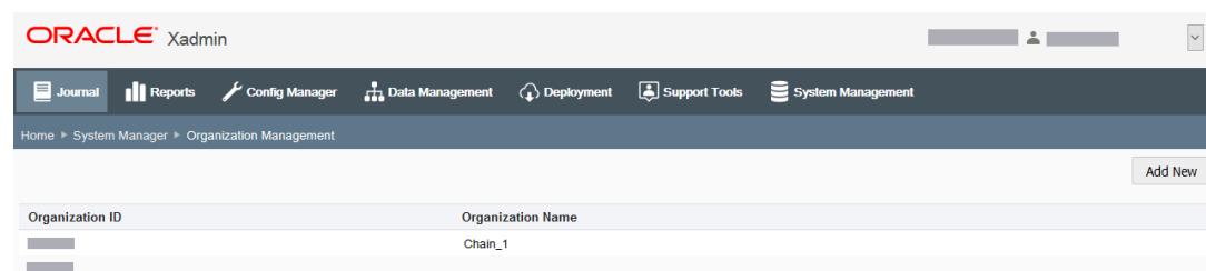
Figure 3-6 Organization Management
