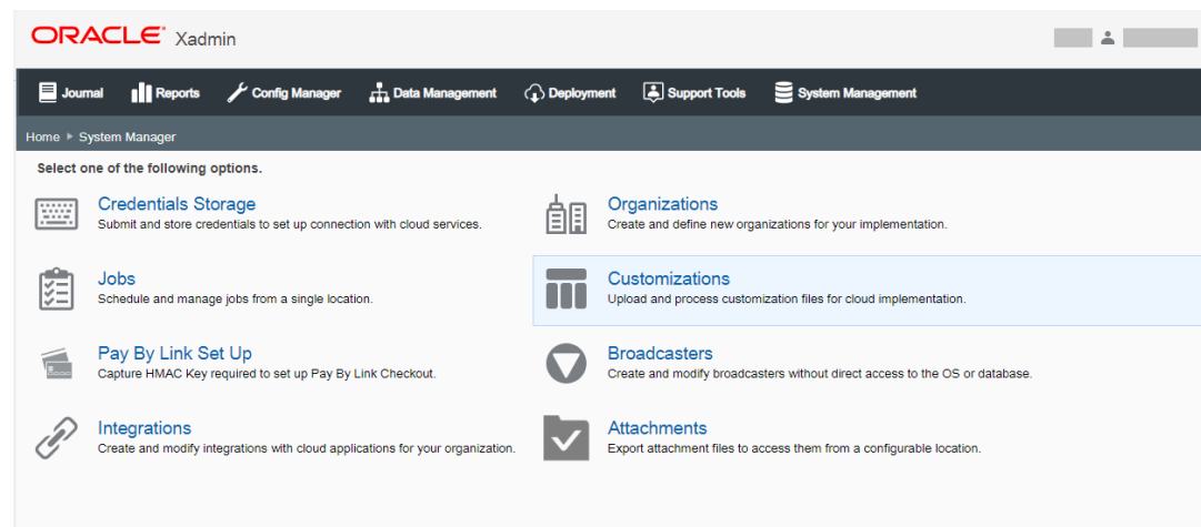
Figure 3-2 System Manager
