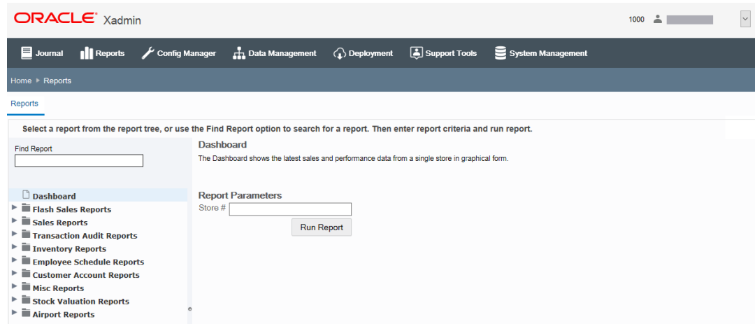
Figure 9-2 Reports - Dashboard
