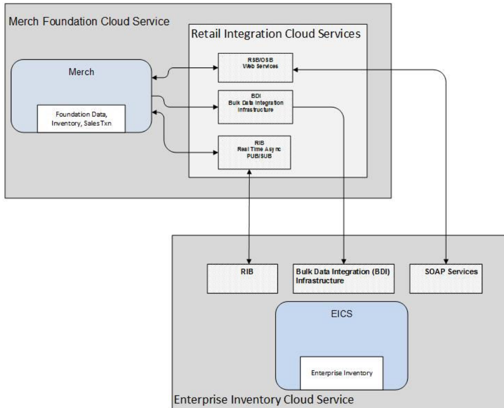
Figure 14-1 Integrations between EICS and MFCS
