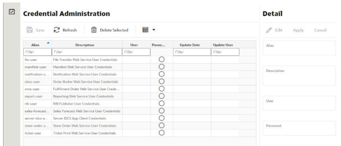
Figure 6-1 Credential Administration
