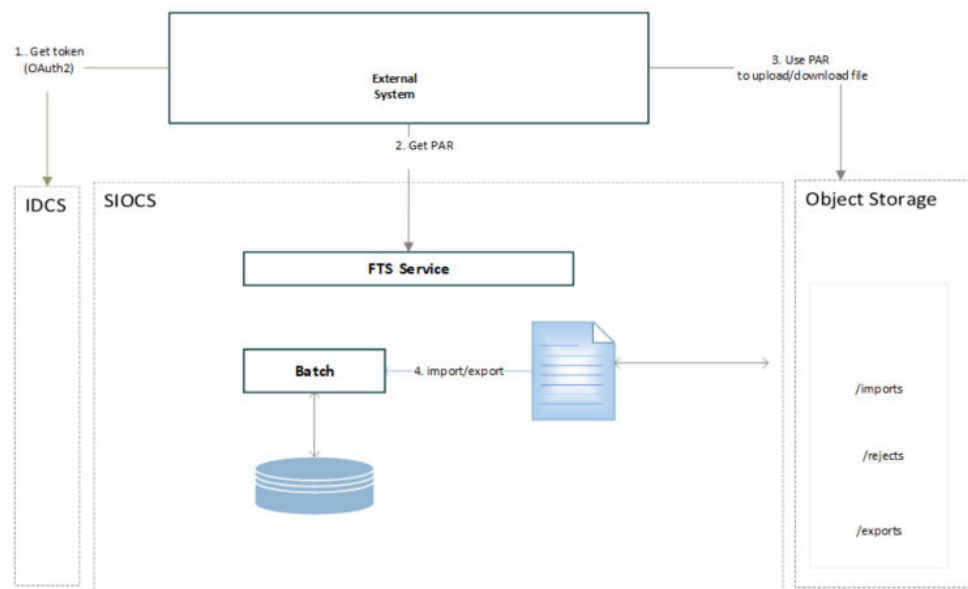
Figure 9-1 File Transfer Service Process Flow
