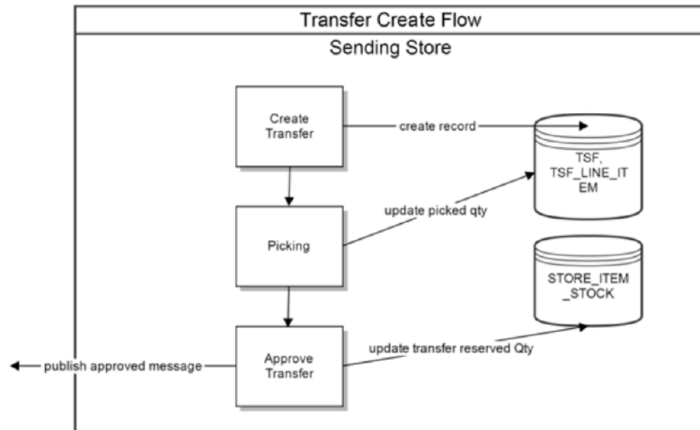
Figure 7-2 Transfer Create Flow
