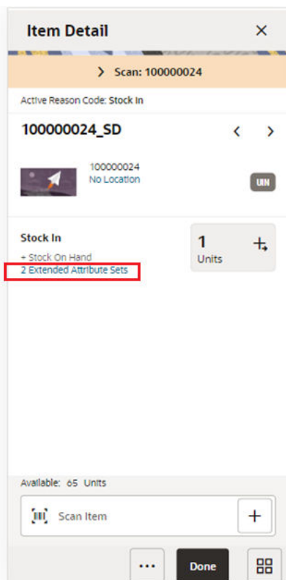
Figure 2-50 Item Detail
