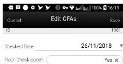
Figure 8-8 Edit CFAs
