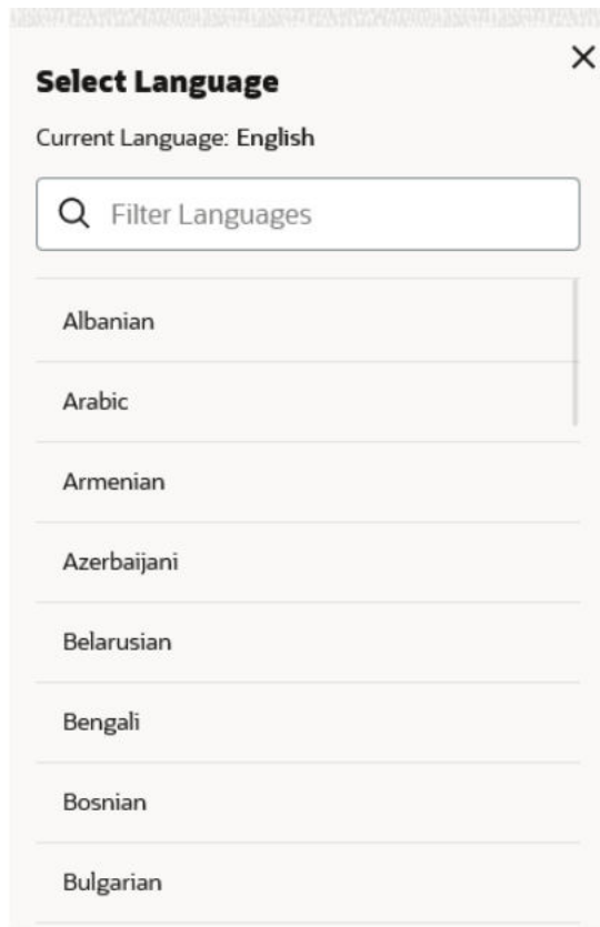
Figure 2-32 Select Language
