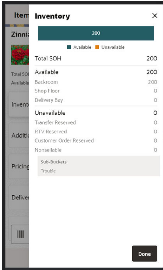
Figure 4-41 Inventory Screen
