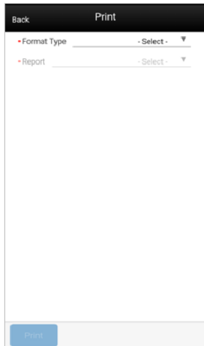
Figure 2-16 Print
