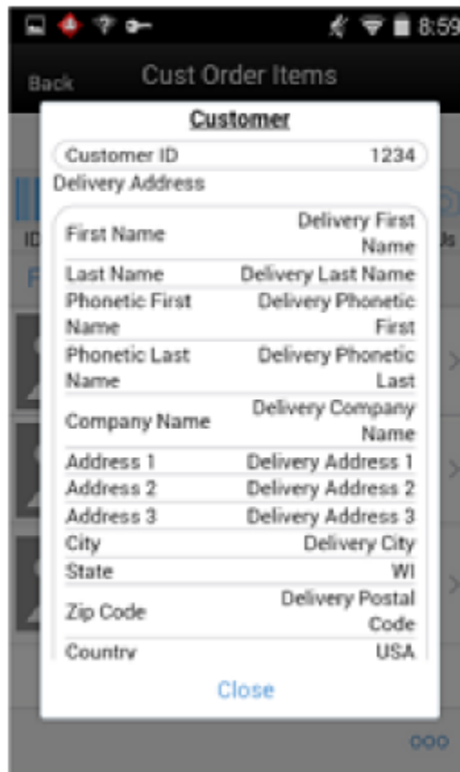
Figure 12-8 Customer Popup
