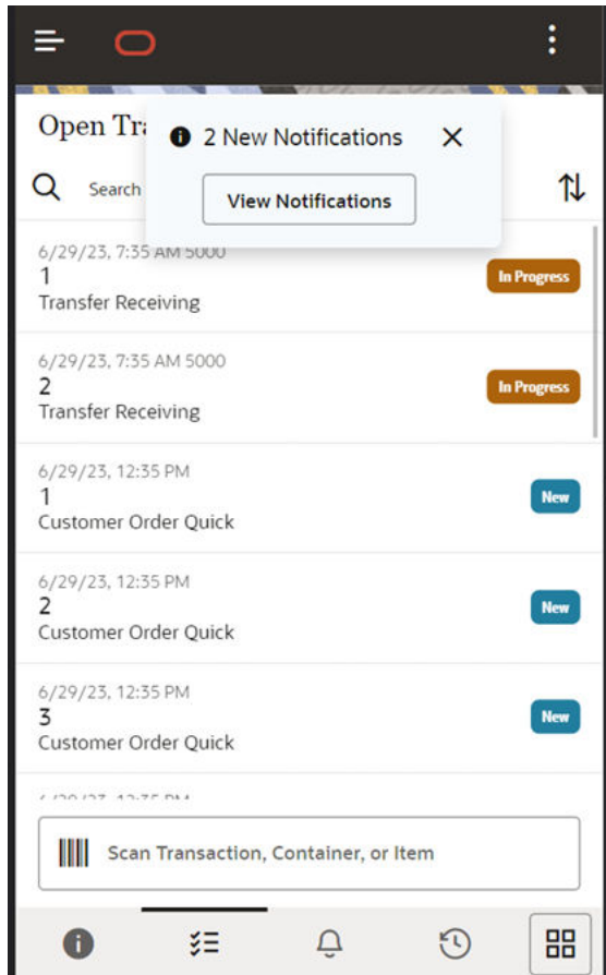
Figure 3-16 Notification Display
