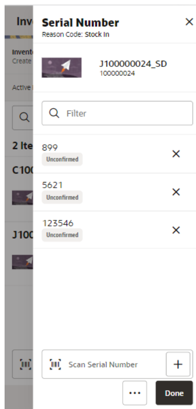
Figure 5-14 UIN Screen
