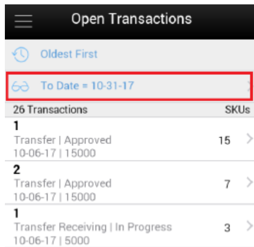
Figure 2-14 Search Criteria
