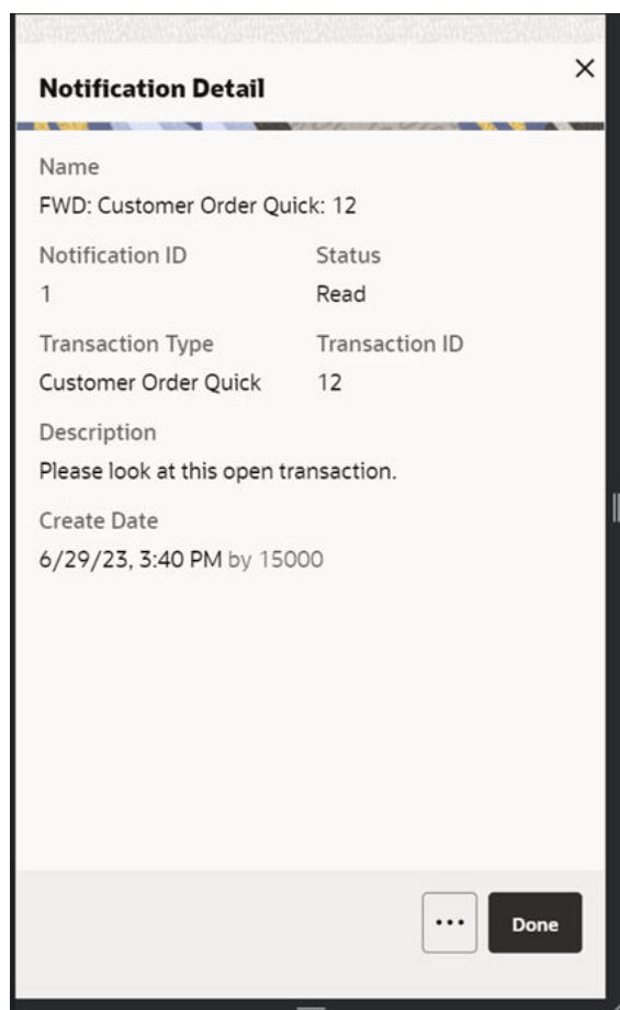
Figure 3-15 Notification Detail
