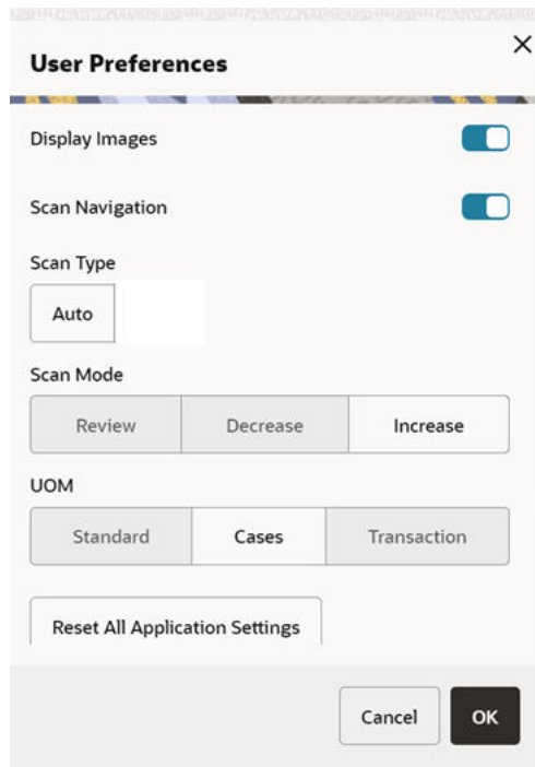
Figure 2-33 Preferences
