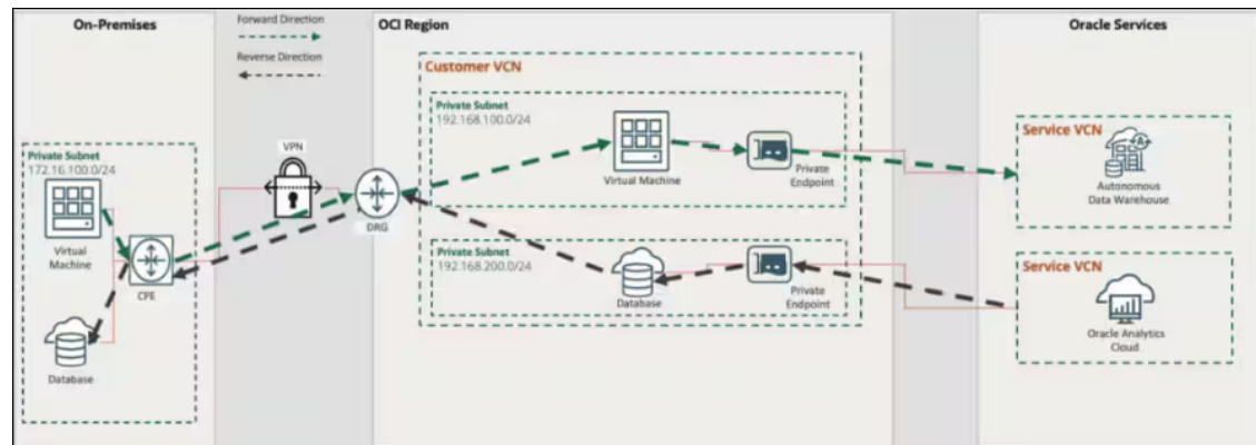
Figure 8-7 Private Endpoints
