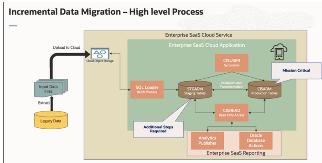
Figure 14-1 Incremental Data Migration - High Leve Process
