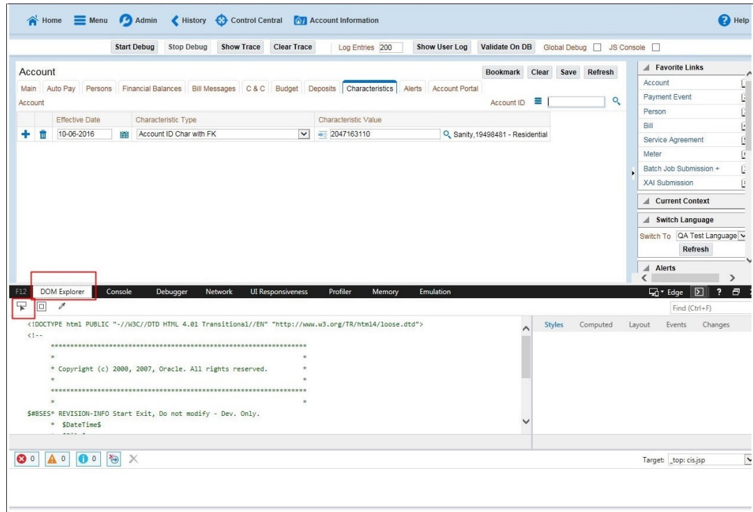
Figure 5-8 DOM Explorer
