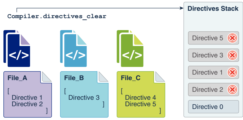
Figure 2-6 Removing All Directives from the Stack
